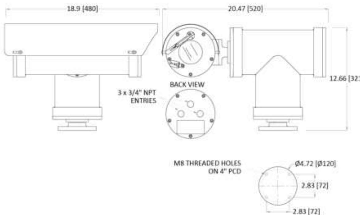
Fig.3 XC40VW Example XC Series unit showing shaft mount fixing points
