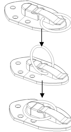
FIG-5.1 Buckle
