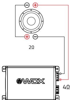
1 X 2Ω DVC SUBWOOFER
