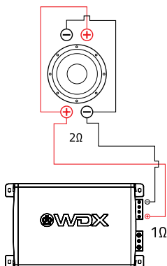
1 X 2Ω DVC SUBWOOFER
