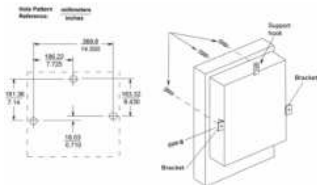
Figure 4: Surface Mounting on a Panel or Wall (Rear View)
