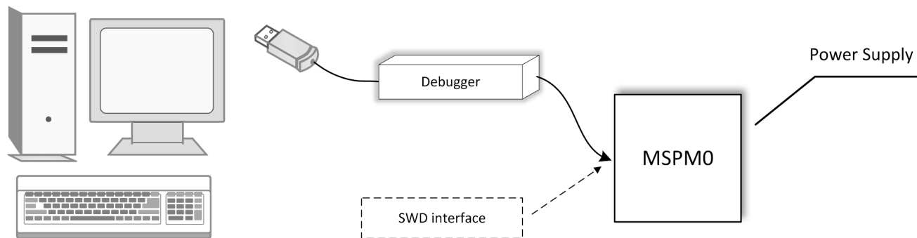
Figure 2-3. MSPM0 Debugging
