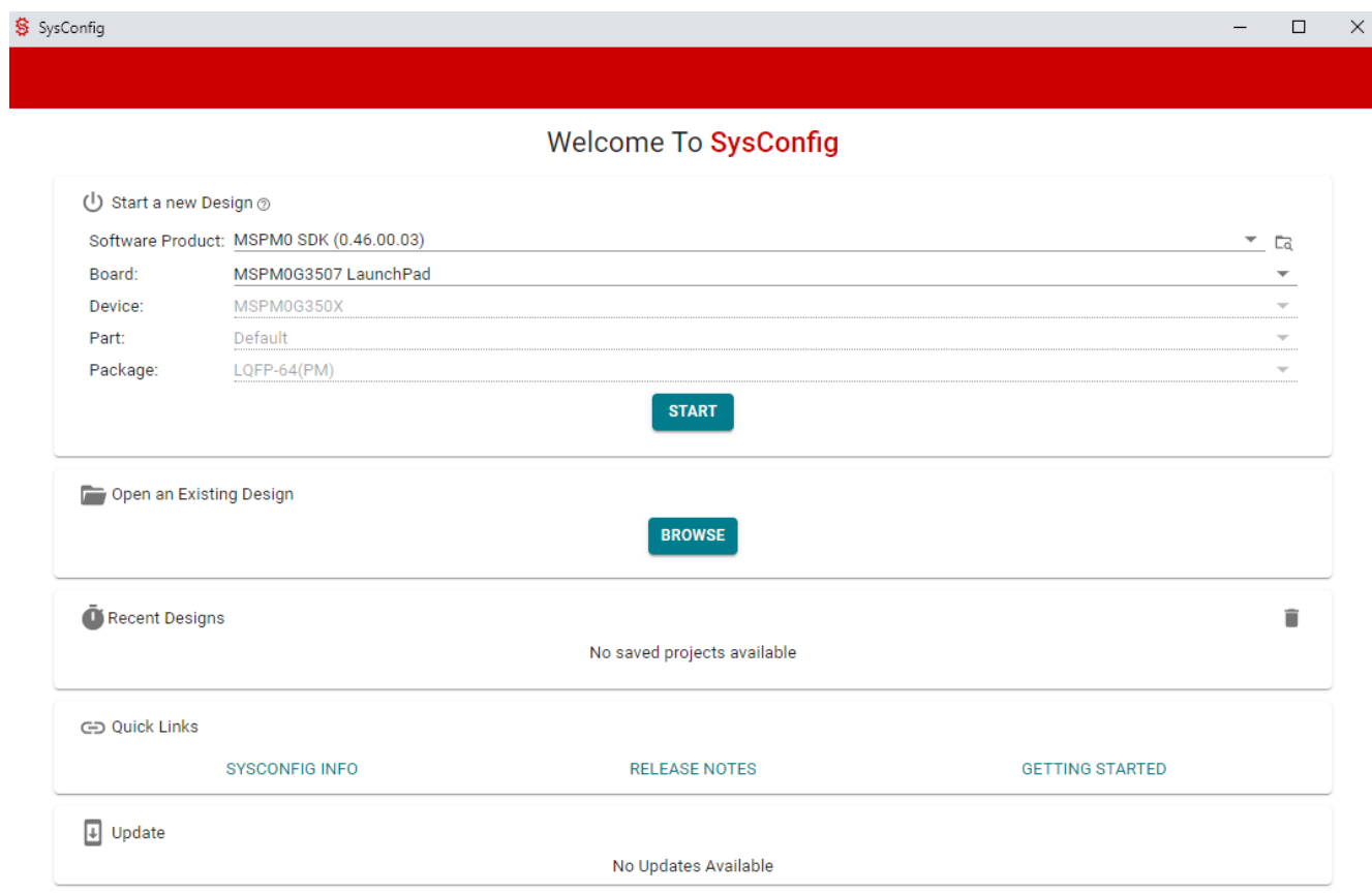
Figure 2-1. MSPM0 SysConfig
