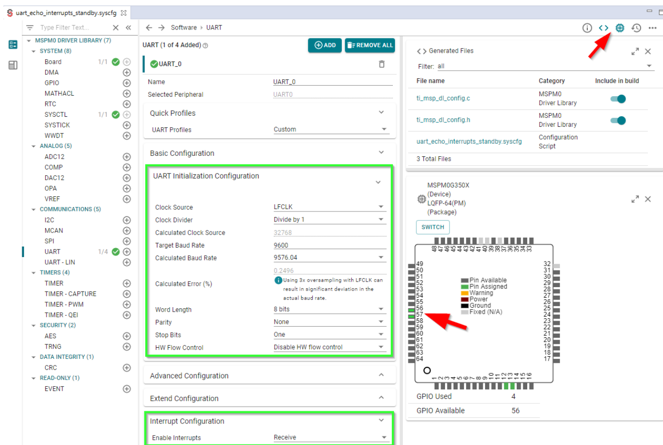
Figure 2-8. UART Configuration
