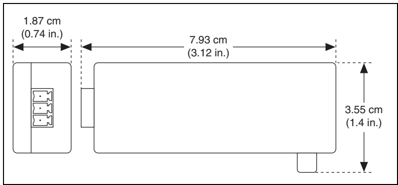
Figure 3. SCC-TC02 Dimensions
