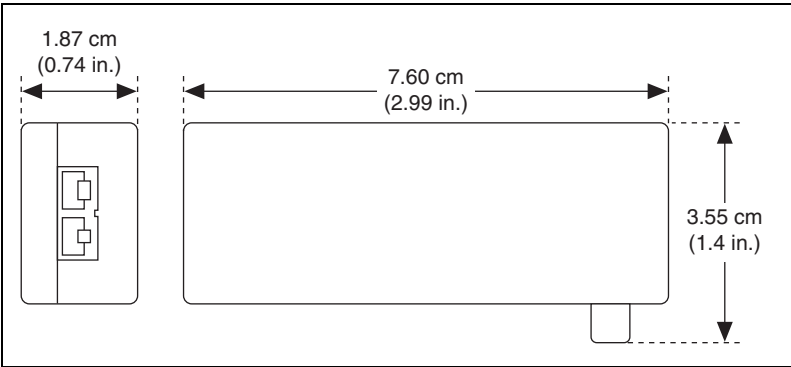
Figure 2. SCC-TC01 Dimensions
