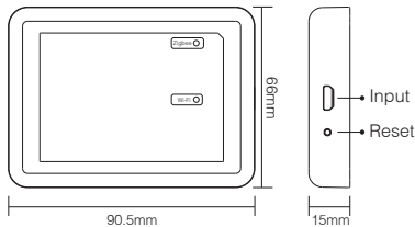
Model No.: ZB-Box1
