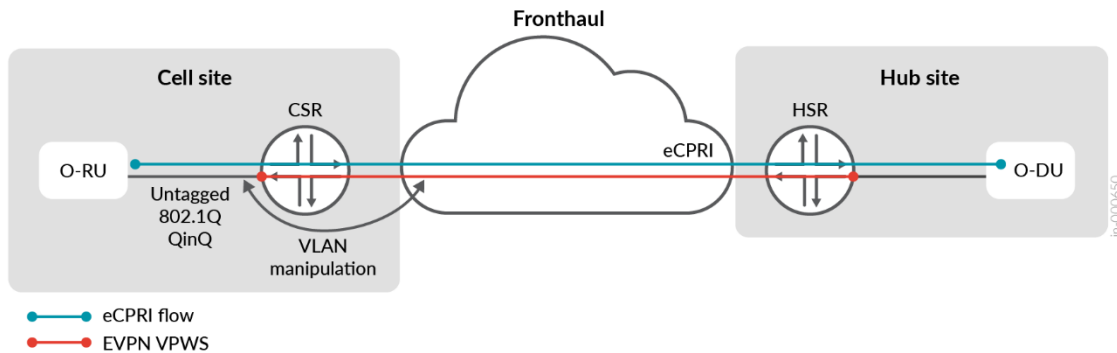
Figure 4: Figure 4. O-RAN Fronthaul Single-Homed EVPN-VPWS/FXC
