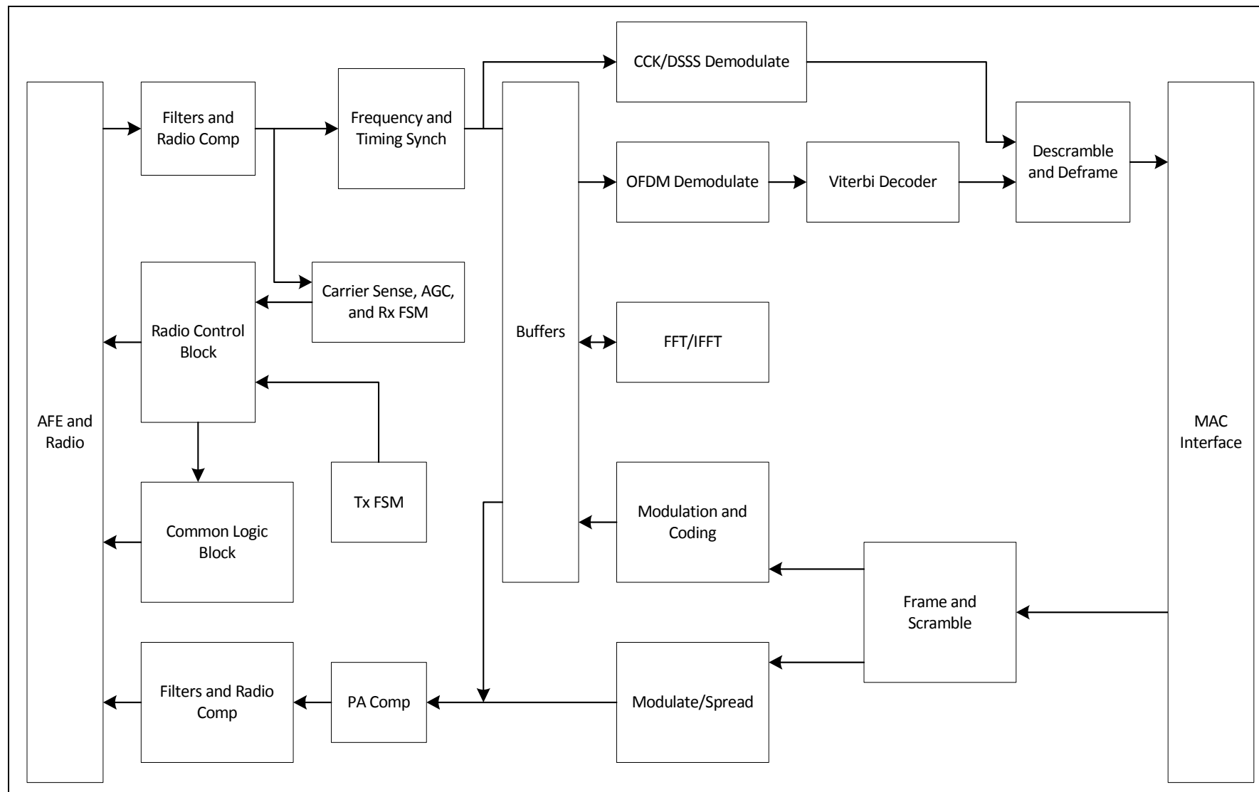
Figure 9: WLAN PHY Block Diagram
