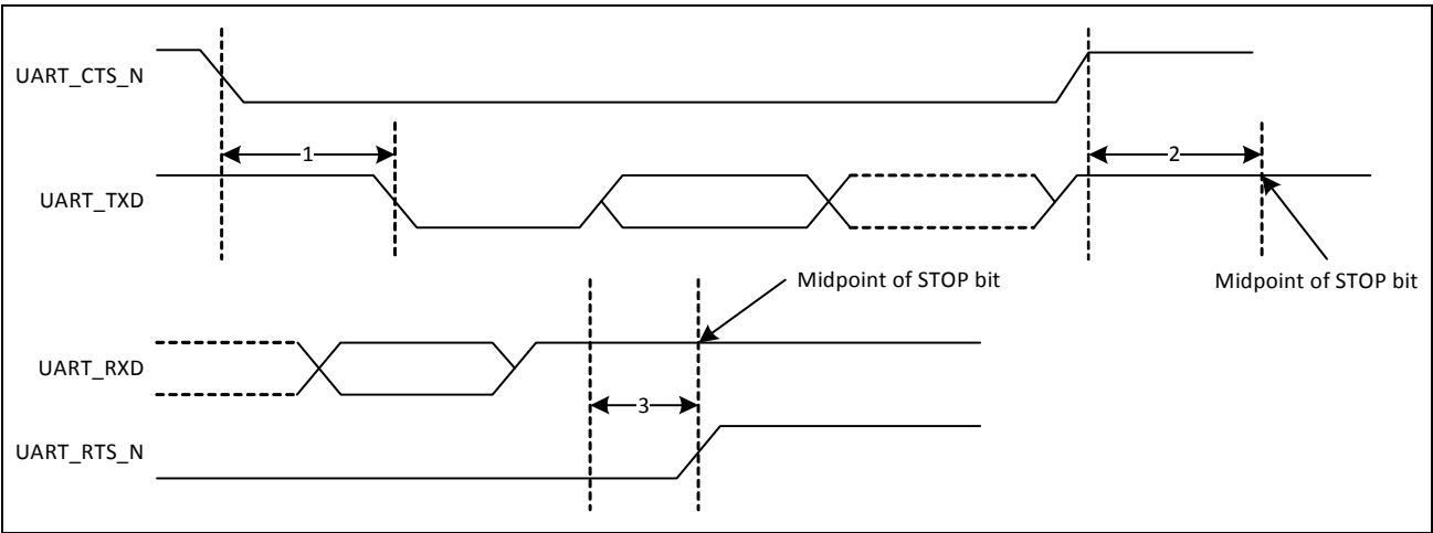
Figure 6: UART Timing
