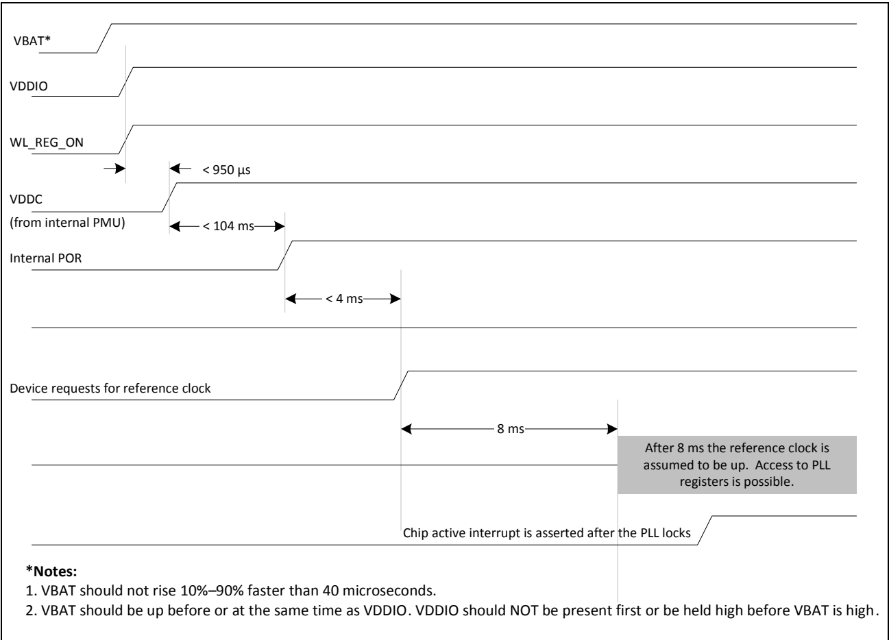
Figure 7: Boot Sequence
