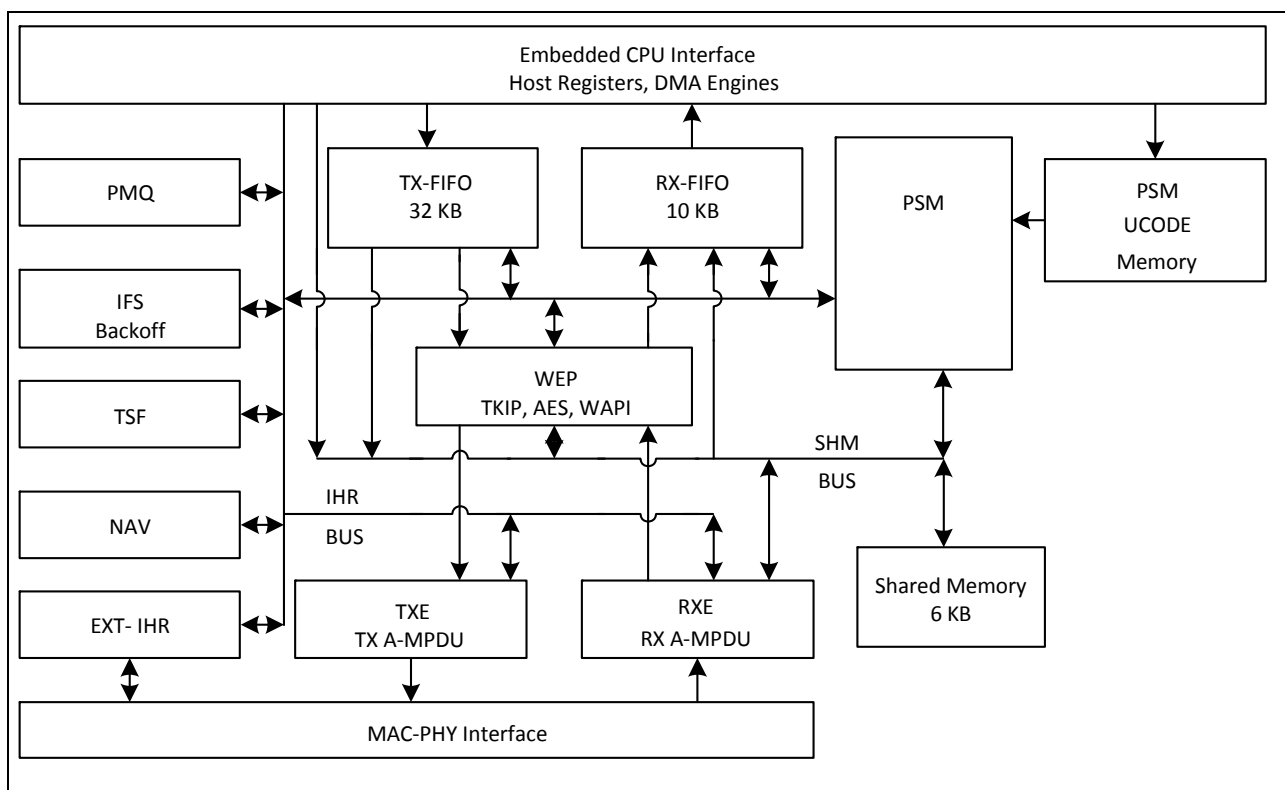
Figure 8: WLAN MAC Architecture
