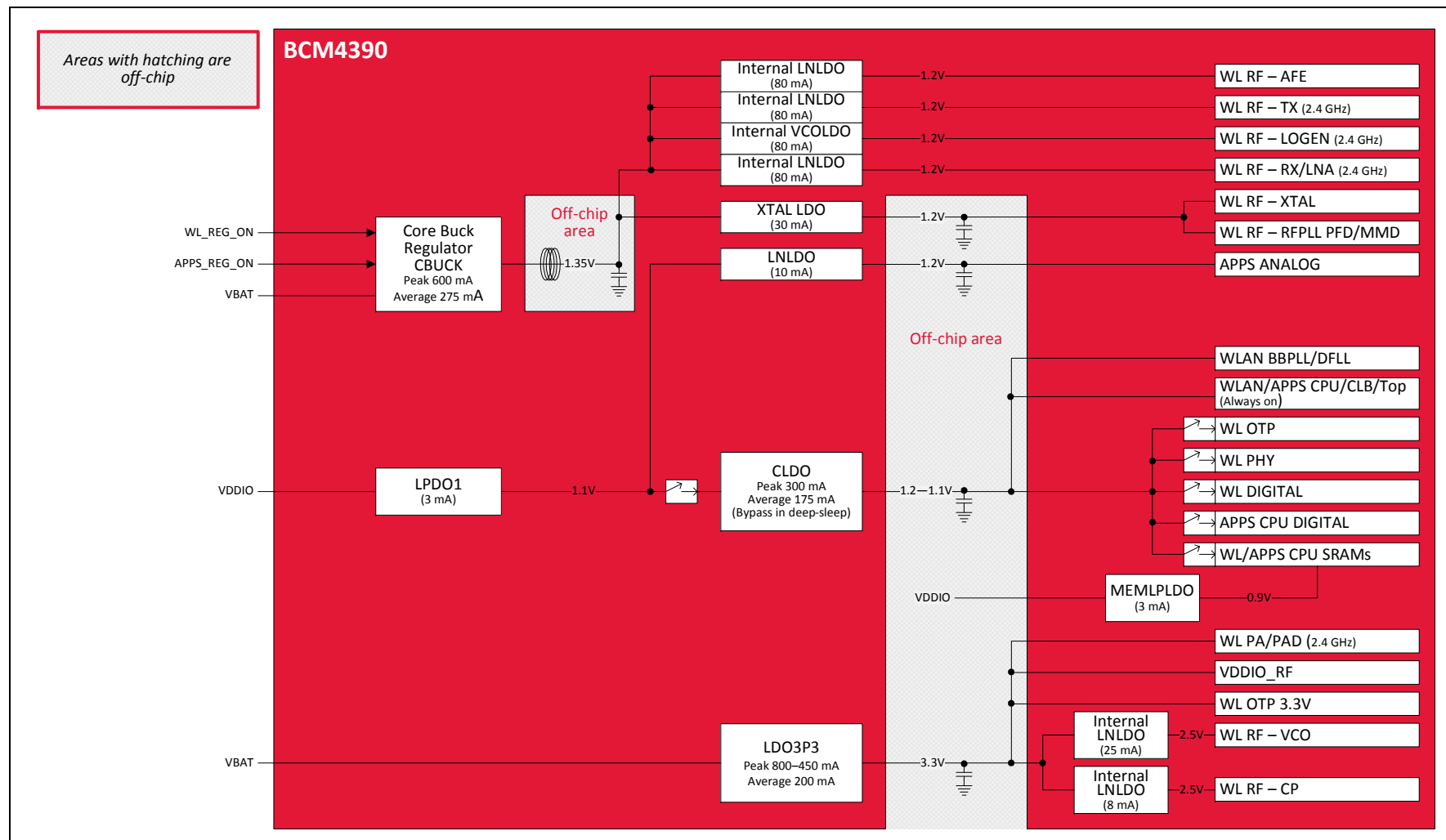
Figure 3: Typical Power Topology
