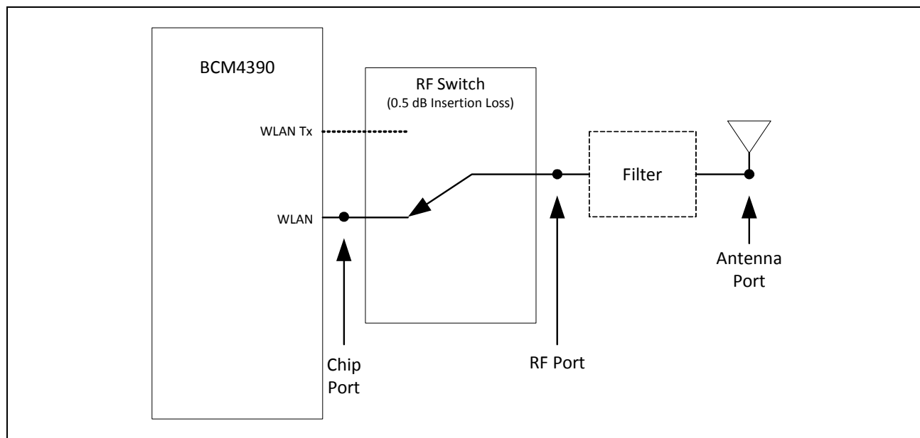
Figure 12: Port Locations
