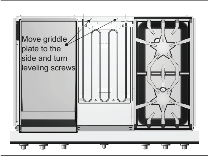
Figure 26: Griddle Plate Leveling Screws
