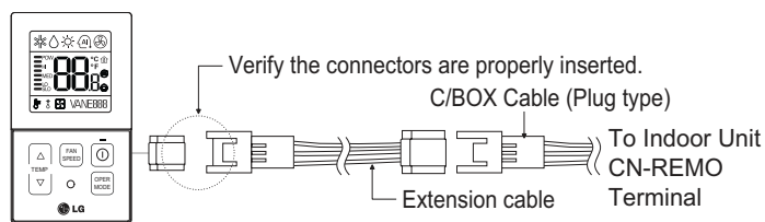
Figure 168: Wired Controller Connections on the Indoor Unit Terminal Block.
