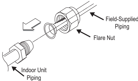
Figure 280: Flare Connection, Side View.
