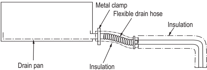
Figure 282:Diagram of an Indoor Unit with a Gravity Drain.
