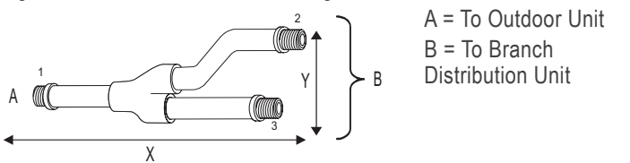
Figure 249:Y-Branch Dimensions Diagram.
