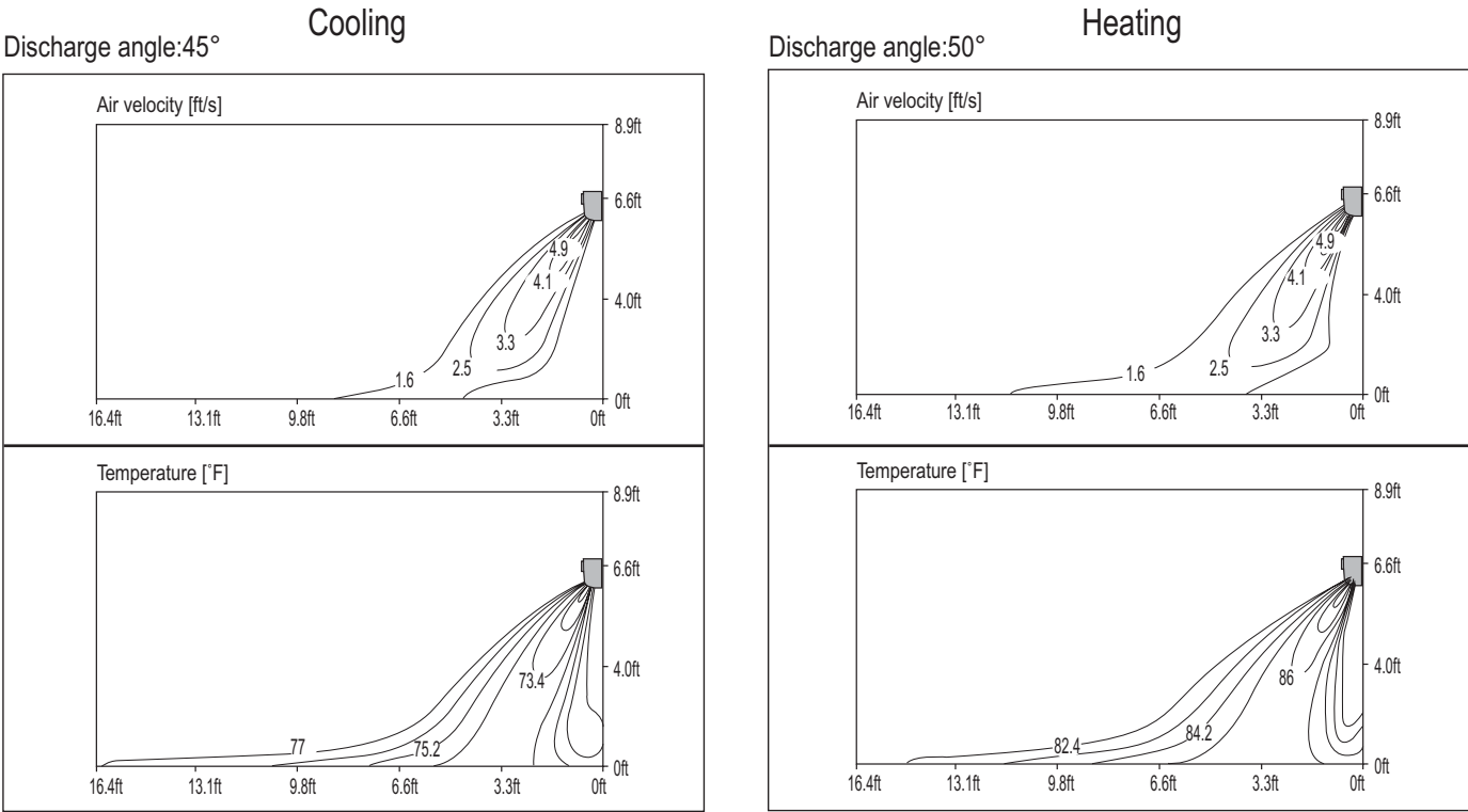
Figure 75:LSN120HSV4 Air Velocity and Temperature Distribution Charts.
