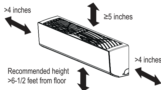
Figure 84: Minimum Clearance Requirements.
