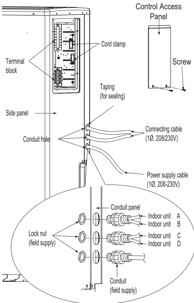
Figure 298: Example of Power Wiring and Communications Cable Terminations.
