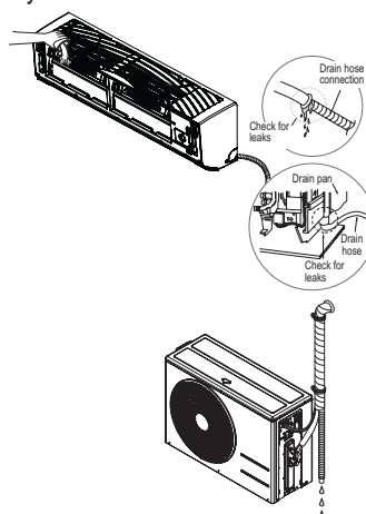
Figure 26: Checking the Drainage System.
