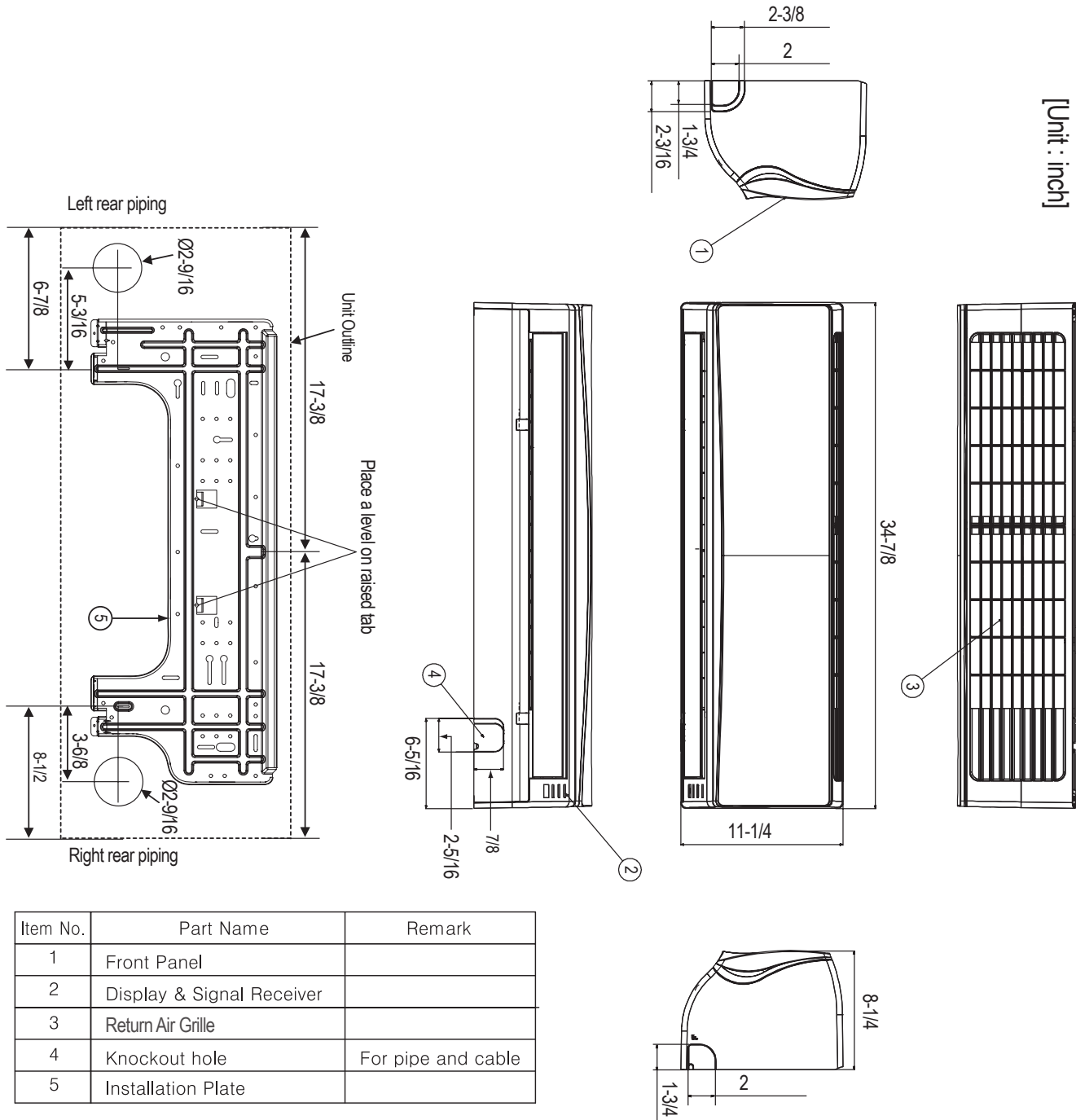
Figure 68: LMN078HVT, LSN090HSV4, LSN120HSV4 and LMN158HVT Dimensions.
