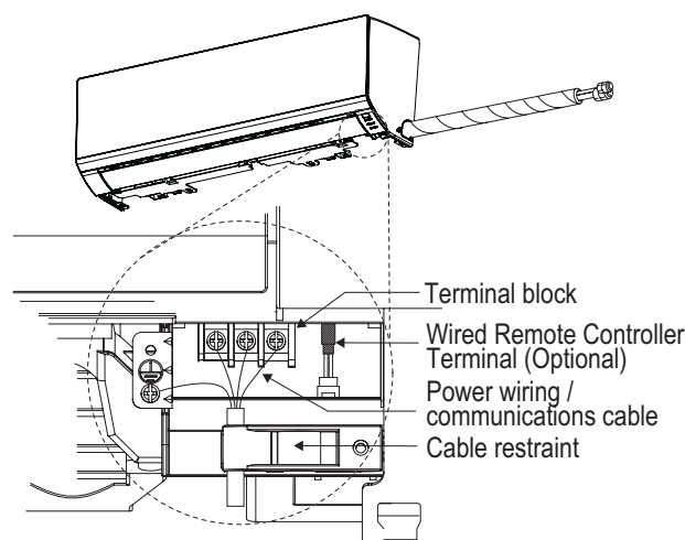
Figure 100: Connecting Power Wiring / Communications Cable.
