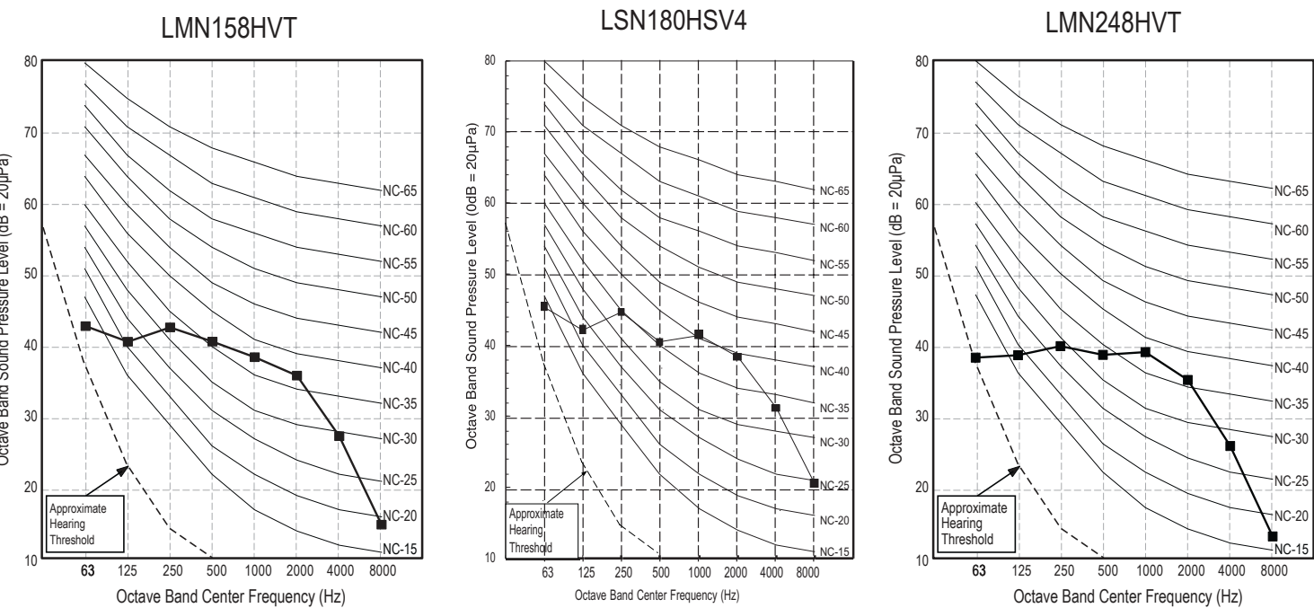
Figure 72:LMN158HVT, LSN180HSV4, and LMN248HVT Sound Pressure Level Diagrams.
