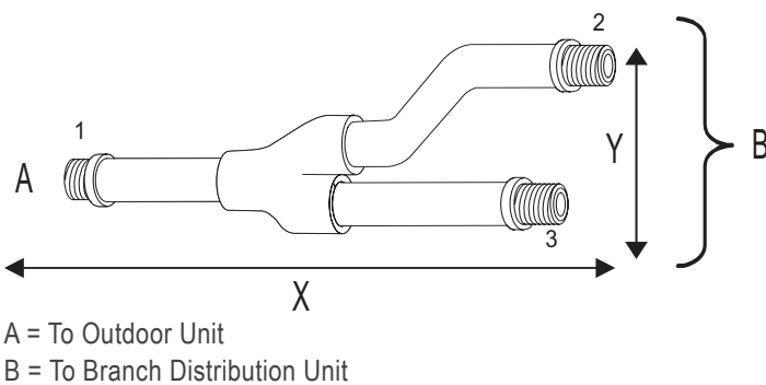
Figure 289:Y-Branch Dimensions Diagram.
