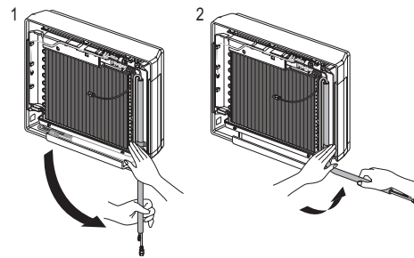
Figure 51: Right Side Piping Access.
