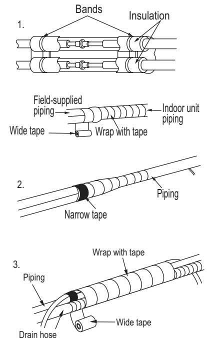
Figure 97: Insulating the Piping.
