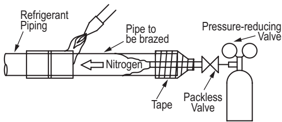
Figure 278: Refrigerant Pipe Brazing.
