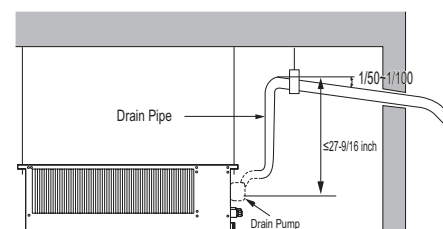
Figure 129: Indoor Unit Using Drain Pump.
