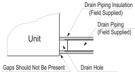
Figure 224: Close up of Drain Piping Connection.
