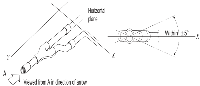
Figure 250:Horizontal Configuration End View.
