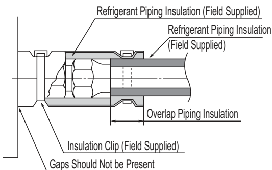
Figure 228: Close Up of Refrigerant Piping Connection Insulation.
