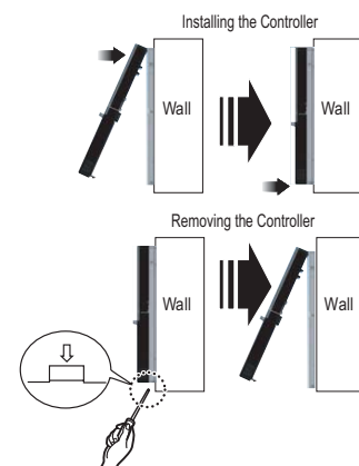
Figure 172: Installing / Removing the Controller.
