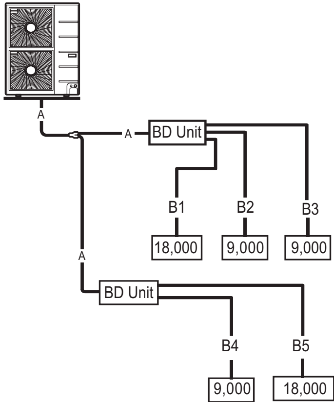
Figure 254:Multi F MAX Additional Refrigerant Charge Example.
