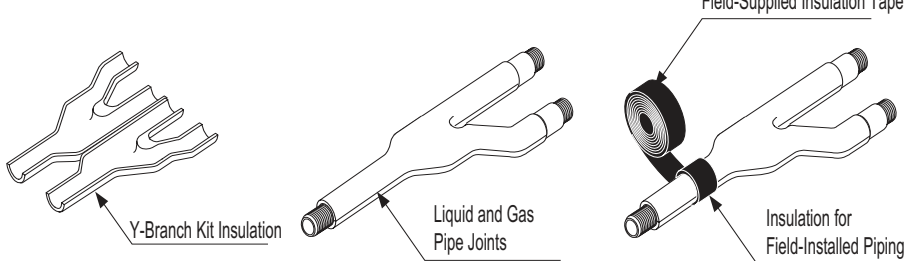
Figure 290:Y-Branch Insulation Jacket Diagram.
