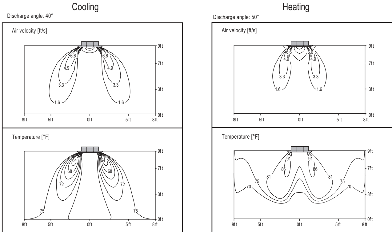
Figure 183:LMCN097HV Air Velocity and Temperature Distribution Charts.
