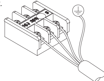
Figure 294: Close up of the Indoor Unit Terminal Block.
