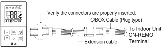
Figure 137:PZCWRC1 LG Wired Remote Extension Cable.
