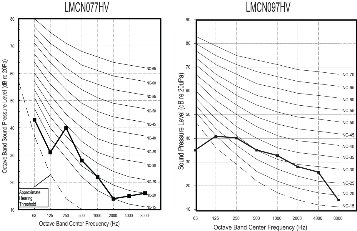
Figure 180: LMCN077HV and LMCN097HV Sound Pressure Level Diagrams.
