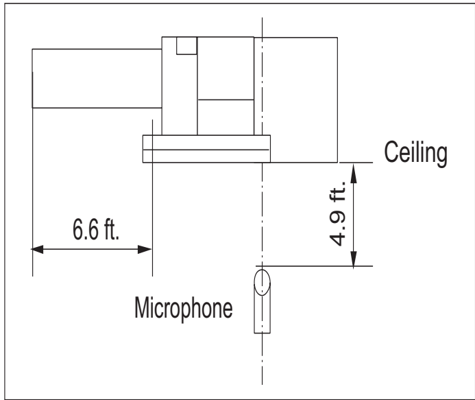
Figure 115: Sound Pressure Level Measurement Location.
