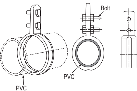
Figure 263:O-Ring Support with Insulation.
