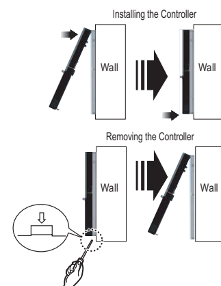
Figure 65:Installing/Removing the Controller.
