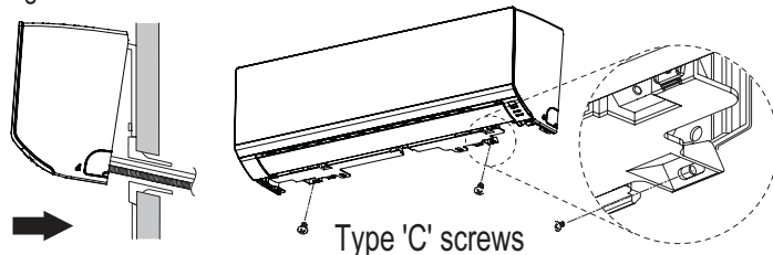
Figure 108: Attach Bottom of Indoor Unit to Installation Plate.
