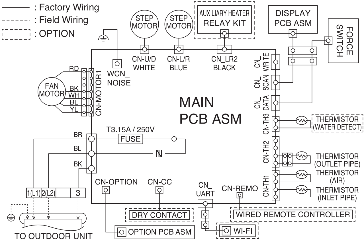
Figure 81: Multi F Standard Wall-Mounted LMN248HVT Indoor Unit Wiring Diagram.
