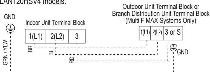
Figure 28: Simplified View of Indoor Unit to Outdoor Unit / Branch Distribution Unit Terminal Connections—LAN090HSV4 and LAN120HSV4 models.
