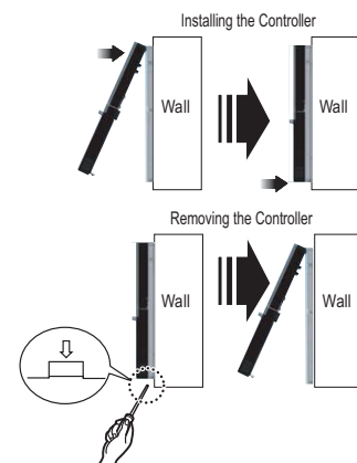
Figure 111: Installing / Removing the Controller.
