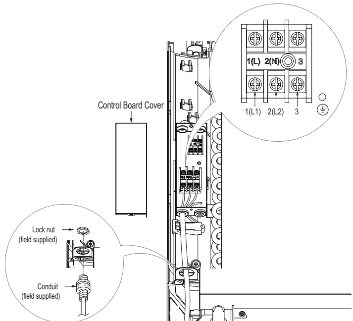
Figure 58: Connecting the Power Wiring / Communications Cable.
