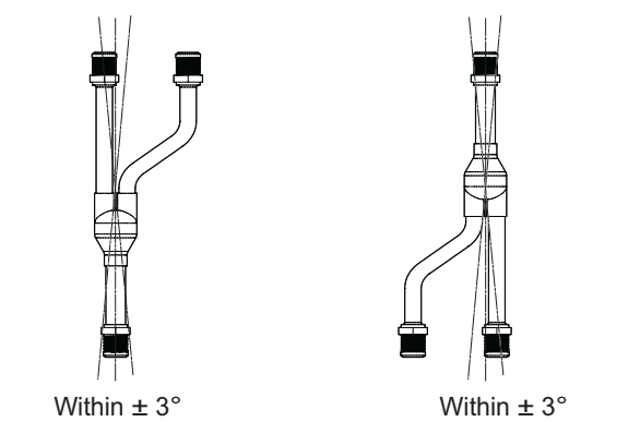
Figure 251:Y-branch Installation Alignment Specification.
