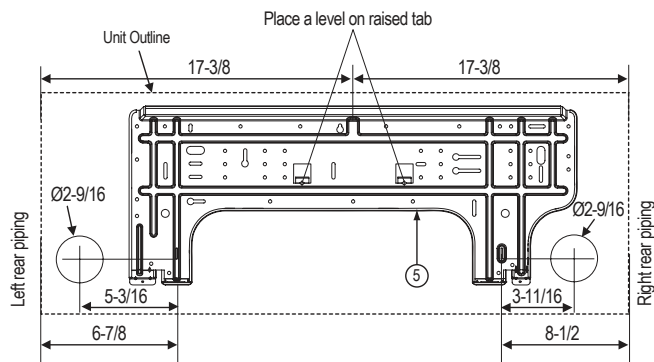
Figure 86: Installation Plate for LMN078HVT, LSN090HSV4, LSN120HSV4, and LMN158HVT Units.
