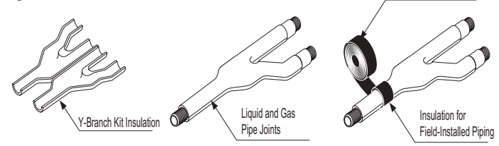
Figure 252:Y-branch Insulation Detail.
