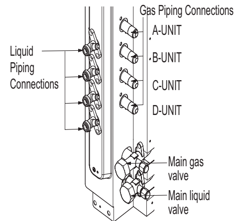
Figure 272: Multi F Refrigerant Pipe Connections (LMU36CHV shown as example).
