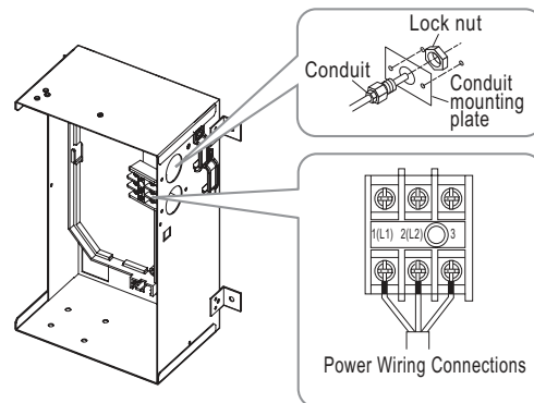
Figure 165: Exterior View of Conduit Installation.
