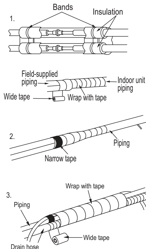
Figure 55: Insulating the Piping.
