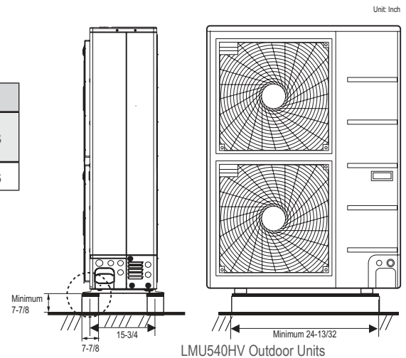
Figure 245: Bolting the Outdoor Unit to the Platform.
