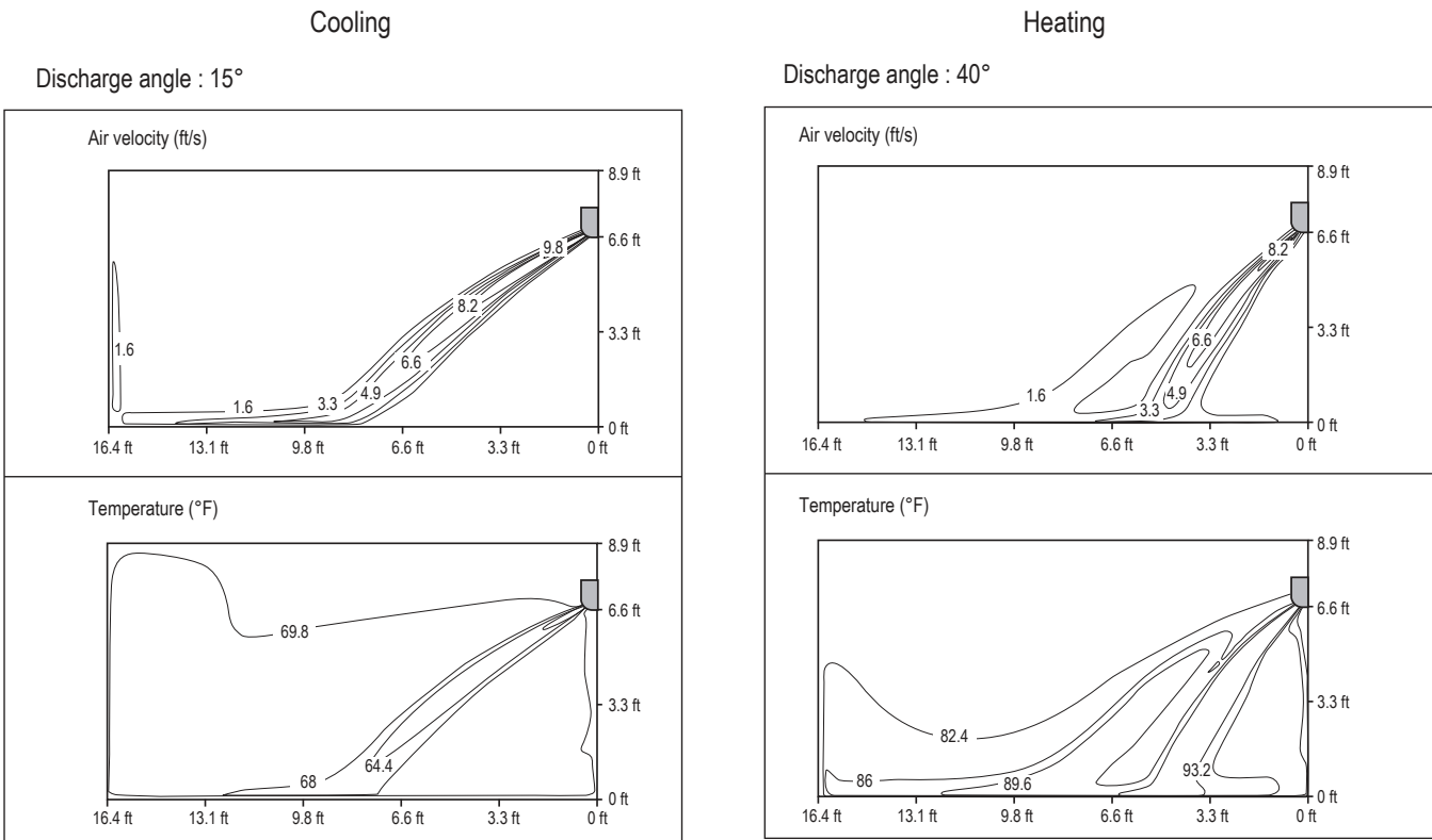
Figure 76:LMN158HVT Air Velocity and Temperature Distribution Charts.
