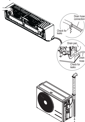
Figure 99: Checking the Drainage System.
