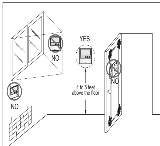
Figure 169: Proper Location for the Wired Controller.
