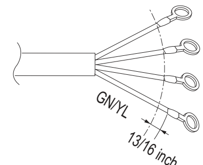
Figure 292: Power Wiring and Communications Cable from the Multi F ODU to the IDUs, or from the Multi F MAX ODU to the BDUs and from the BD Unit to the IDUs.
