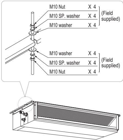
Figure 127:Hanging the Indoor Unit.
