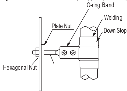
Figure 267:One-Point Down-Stop Support (>441 lbs.).
