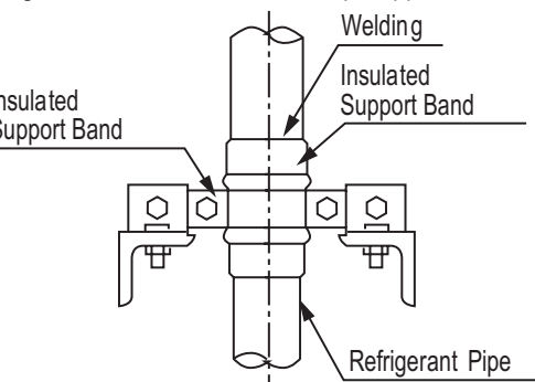
Figure 268:Two-Point Down-Stop Support.
