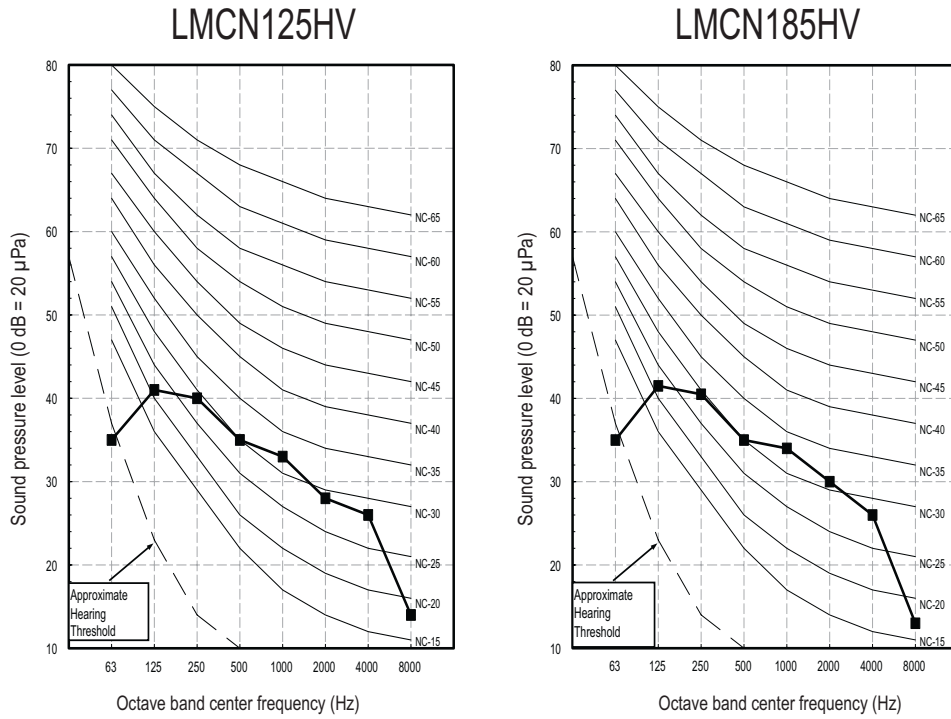
Figure 181: LMCN125HV and LMCN185HV Sound Pressure Level Diagrams.
