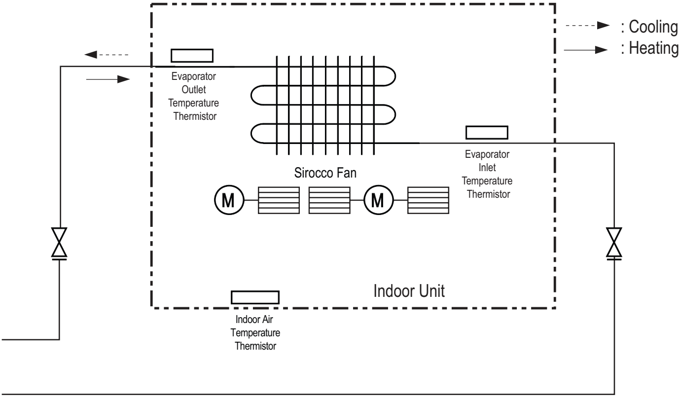
Figure 118:LMDN126HV and LMDN186HV Refrigerant Flow Diagram.
