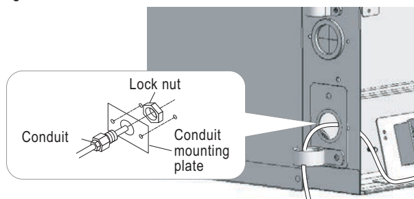
Figure 135: Exterior View of Conduit Installation.
