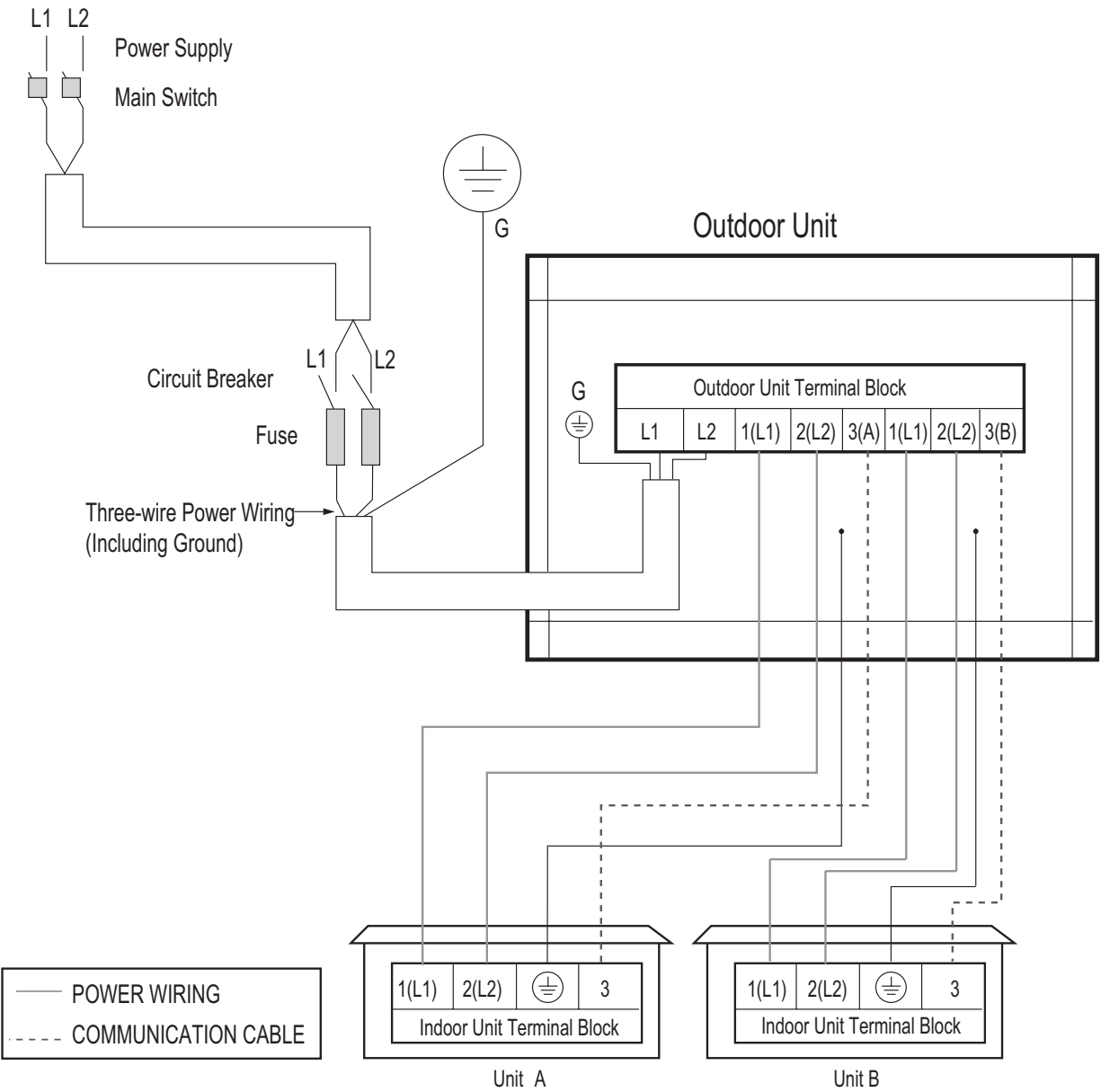
Figure 299: Multi F LMU18CHV System Power Wiring and Communications Cable.
