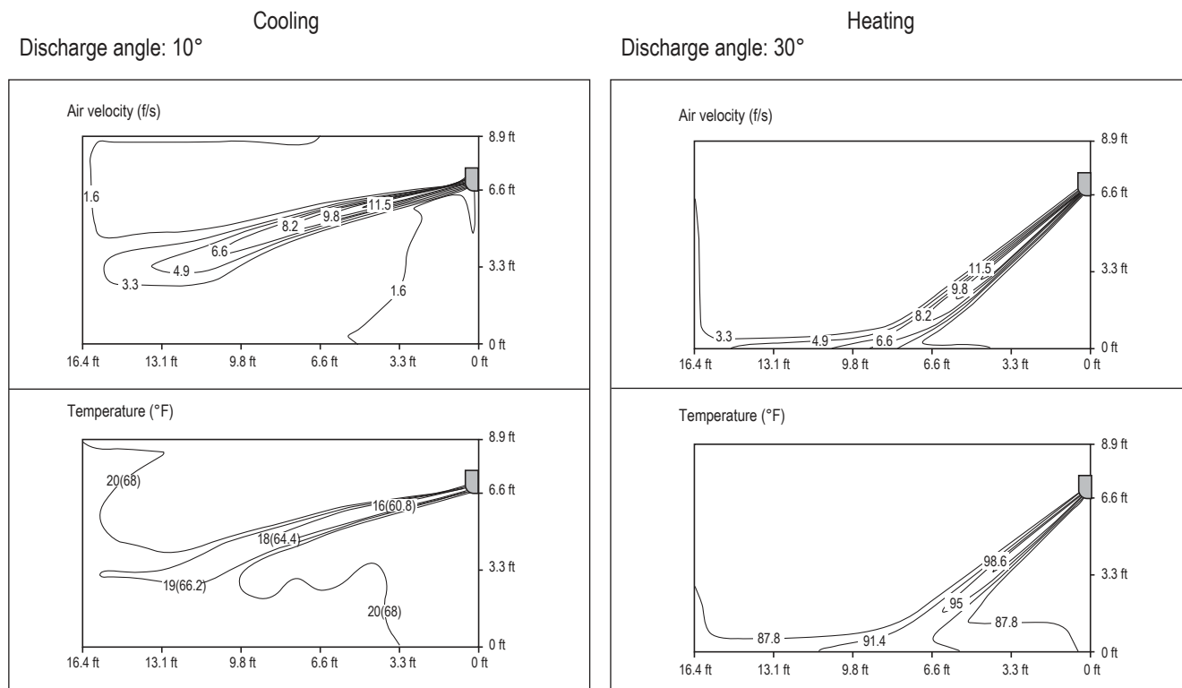
Figure 78: LMN248HVT Air Velocity and Temperature Distribution Charts.
