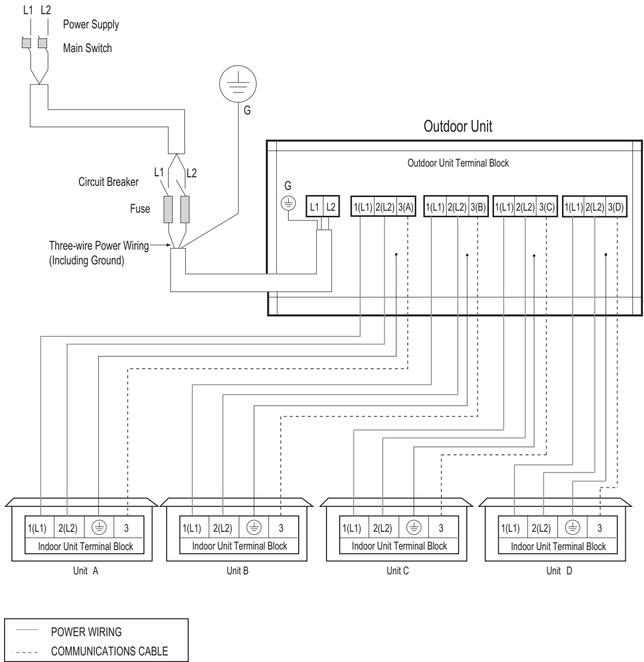
Figure 301:Multi F LMU36CHV System Power Wiring and Communications Cable.
