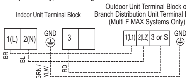
Figure 134: Indoor Unit to Outdoor Unit / Branch Distribution Unit (Multi F MAX systems only) Power Wiring / Communications Cable Connections.
