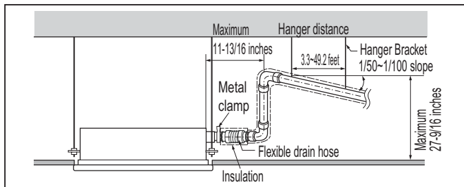
Figure 159: Drain Piping Installation Dimensions.
