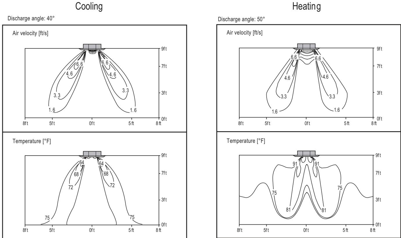
Figure 185:LMCN185HV Air Velocity and Temperature Distribution Charts.
