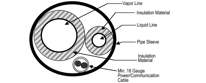
Figure 270:Typical Arrangement of Refrigerant Pipe and Cable(s) in a Utility Conduit.
