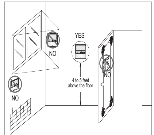
Figure 107:Proper Location for the Wired Controller.
