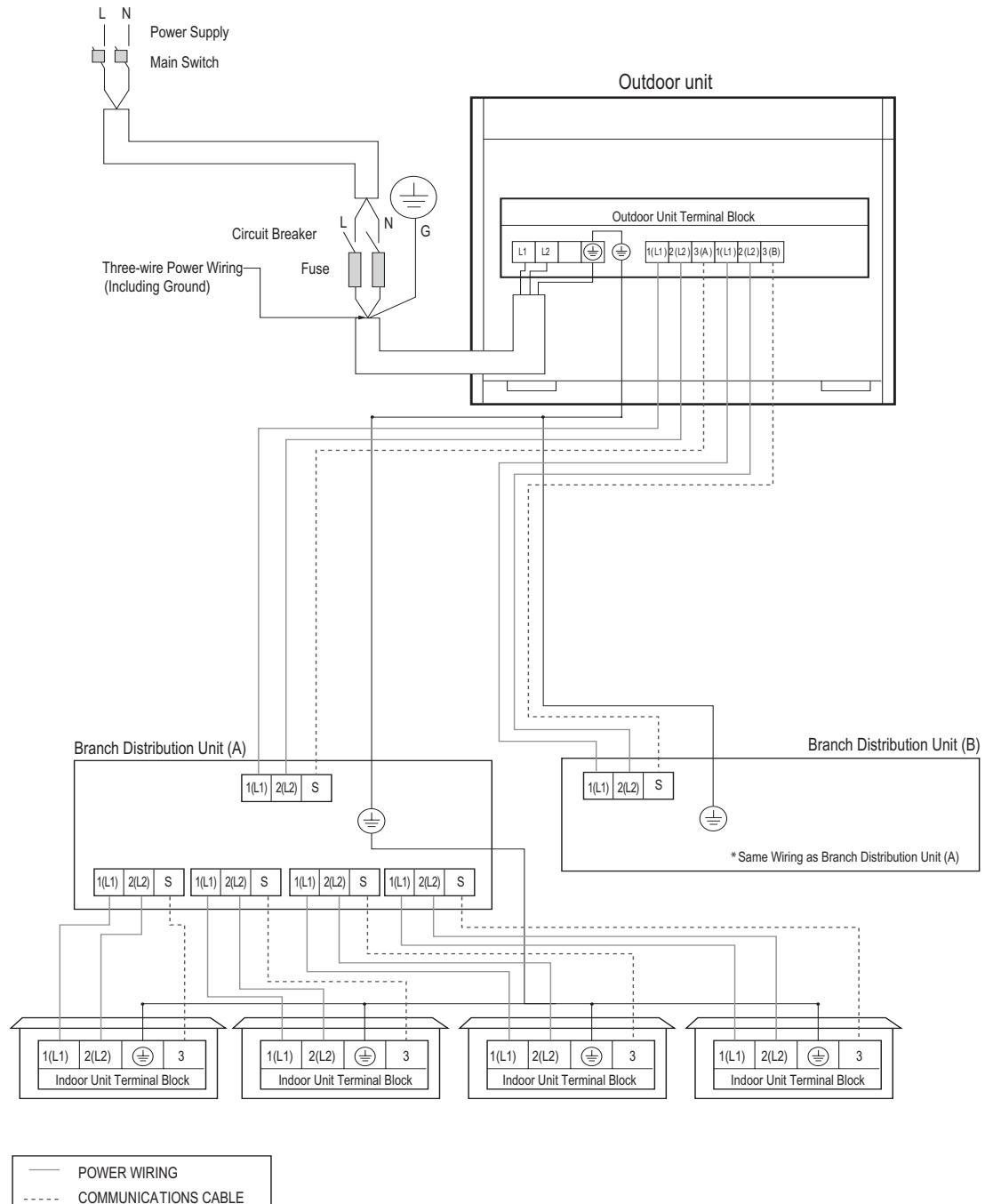
Figure 302: Multi F MAX LMU540HV System Power Wiring and Communications Cable.
