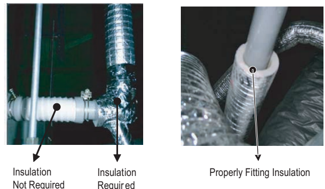
Figure 287: Properly Insulating the Drainage Piping.
