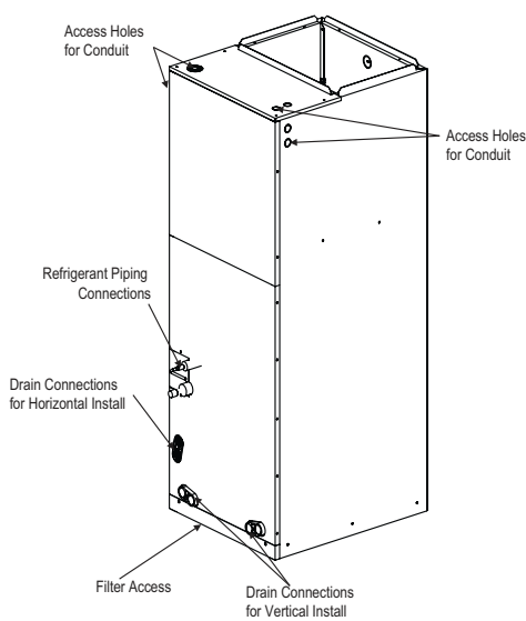
Figure 217: General and Duct Connection Dimensions.
