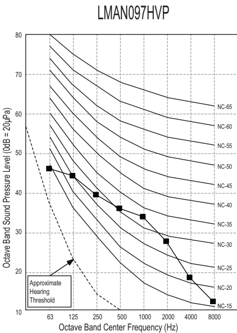
Figure 40: Sound Pressure Level Diagrams.
