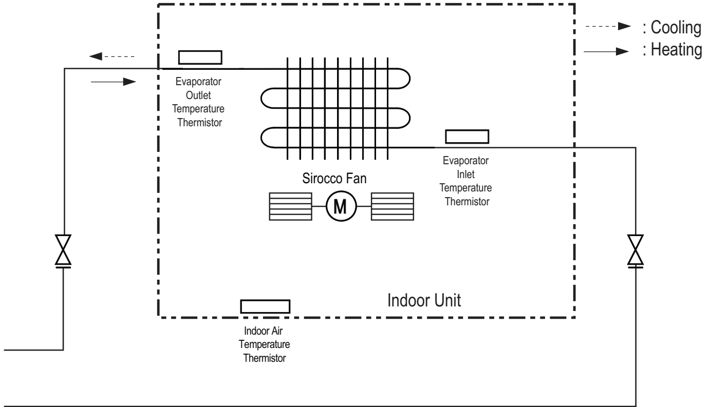
Figure 117: LMDN096HV Refrigerant Flow Diagram.
