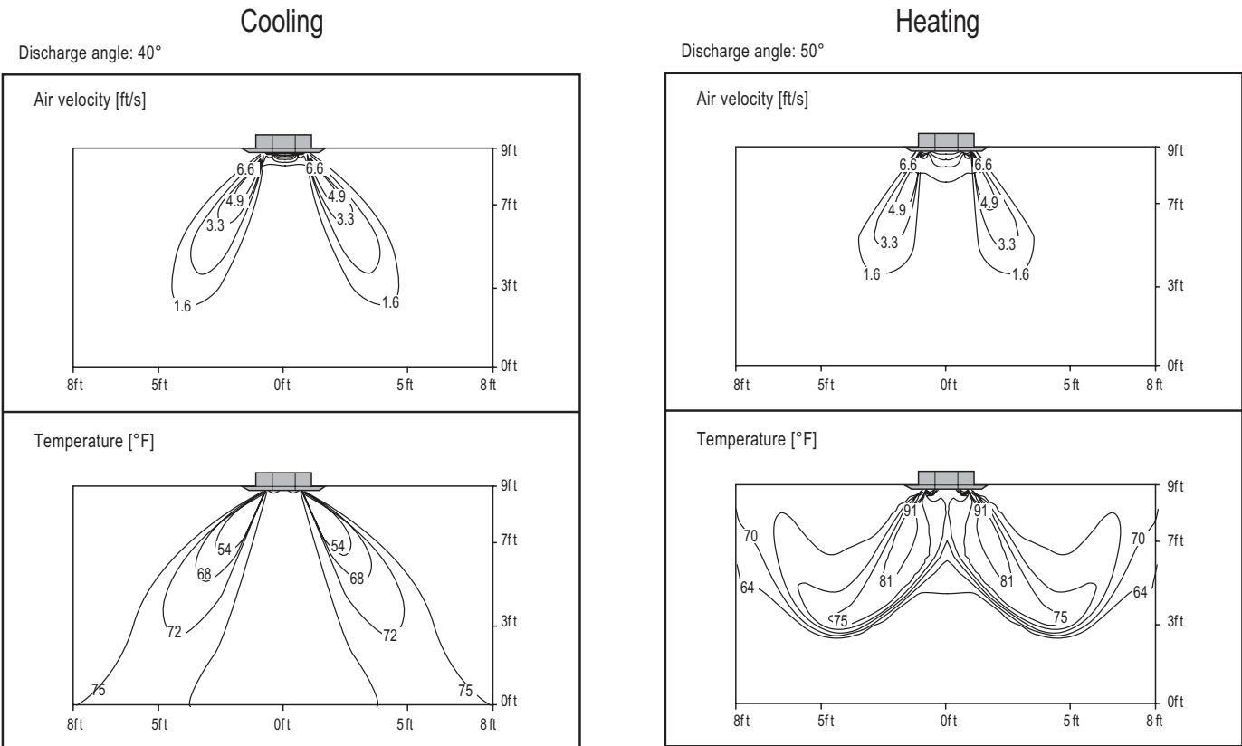
Figure 183:LMCN097HV Air Velocity and Temperature Distribution Charts.
