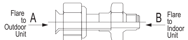
Figure 273: Connection Socket Diagram.
