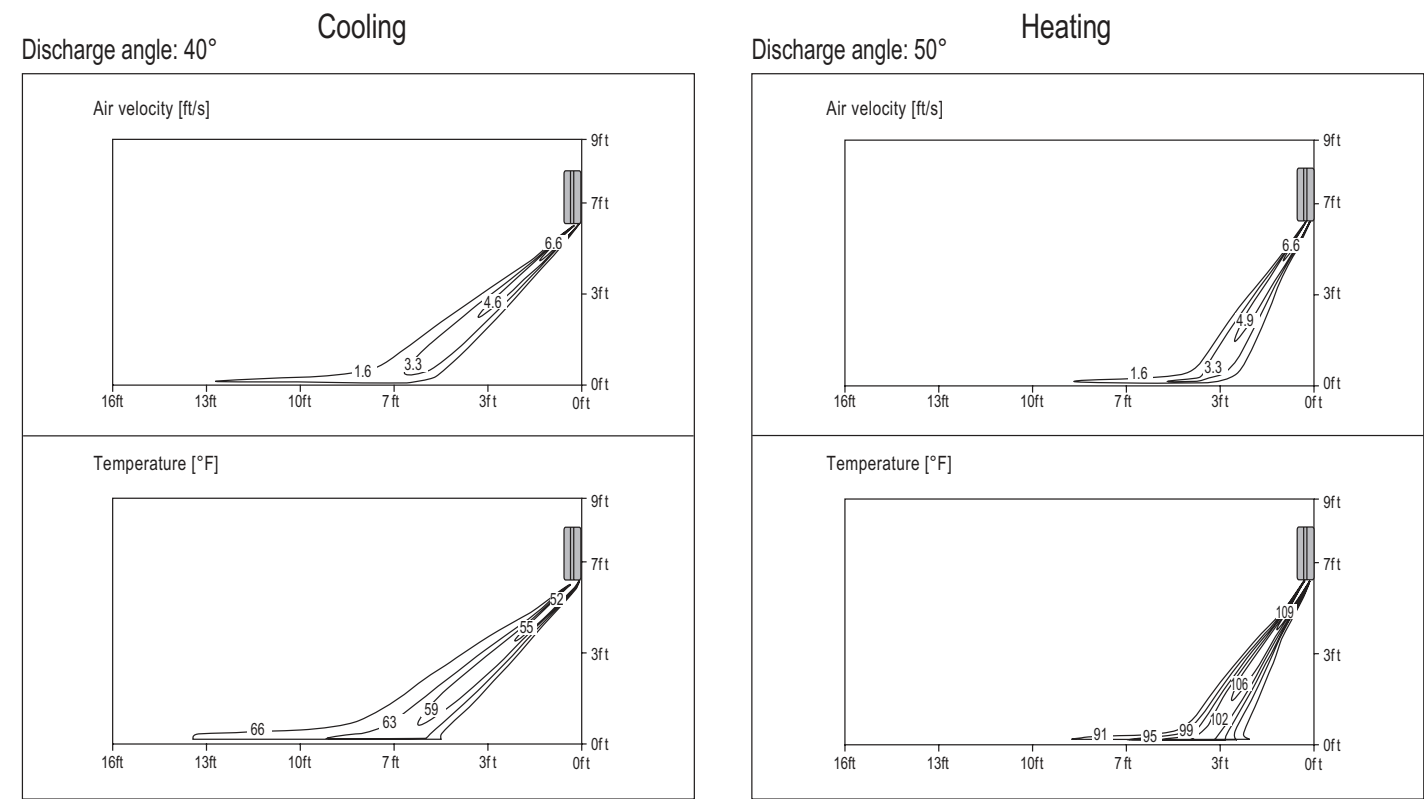
Figure 41: LMAN097HVP Air Velocity and Temperature Distribution Charts.
