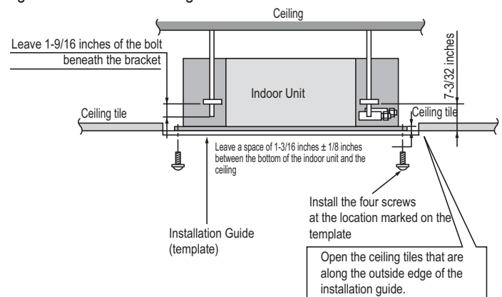
Figure 193: Installation Diagram.
