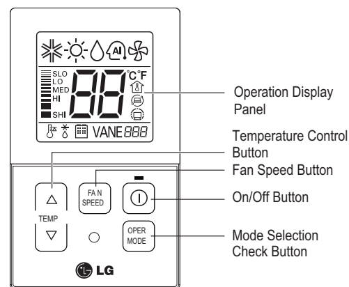
Figure 166: AKB72955816 1 Wired Controller.
