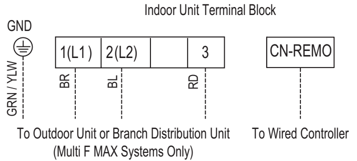
Figure 106:Wired Controller Connection on Indoor Unit Terminal Block—LSN180HSV4 and LMN248HVT Models.
