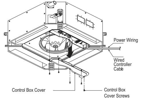
Figure 198: Power Wiring and Communications Cable Connection Access.
