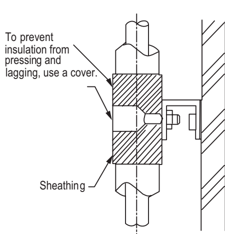
Figure 265:U-Bolt Support with an Insulated Pipe.
