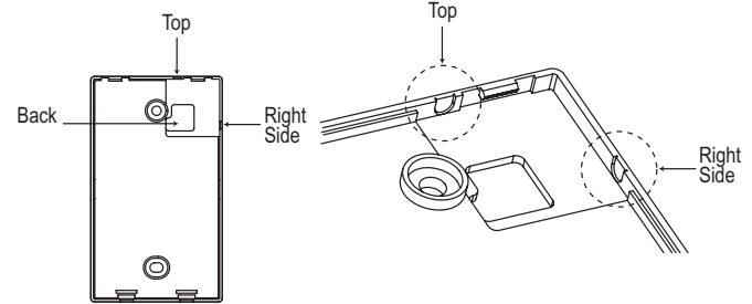
Figure 205: Attaching the Wall Plate.
