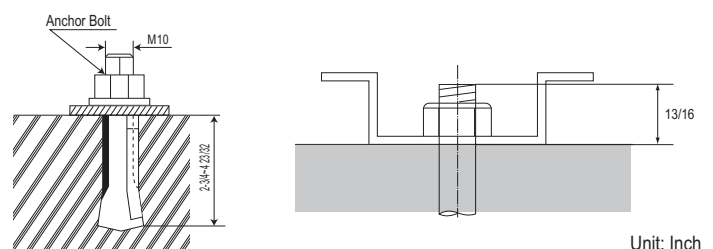
Figure 246: Close up of Bolt Attachment.
