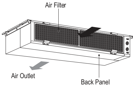
Figure 122:Air inlet from the back of the indoor unit.
