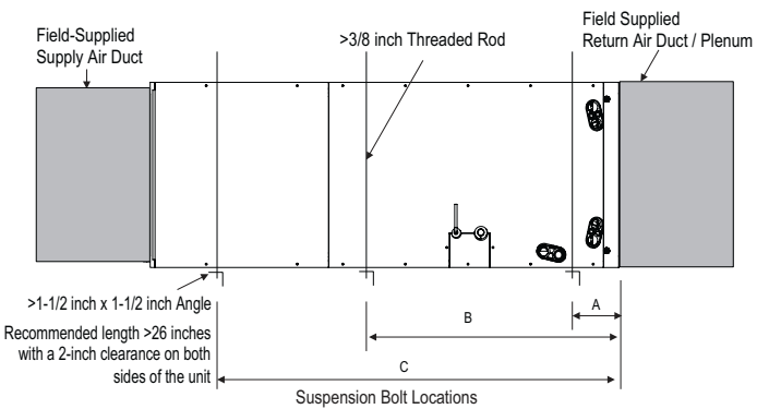
Figure 220:Horizontal Installation.
