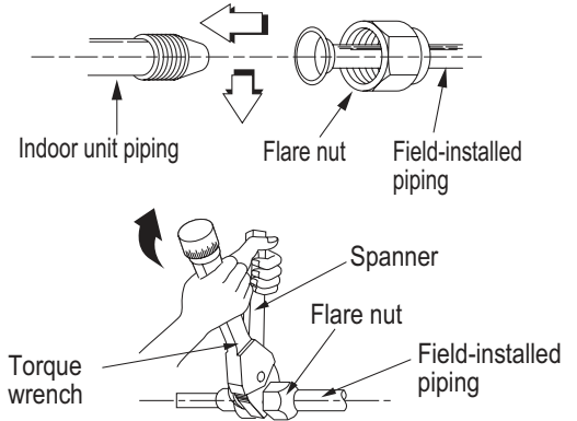
Figure 95: Indoor Unit to Field-Installed Piping Connection.
