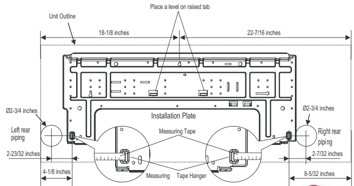
Figure 14: Installation Plate for LAN180HSV4 Units.
