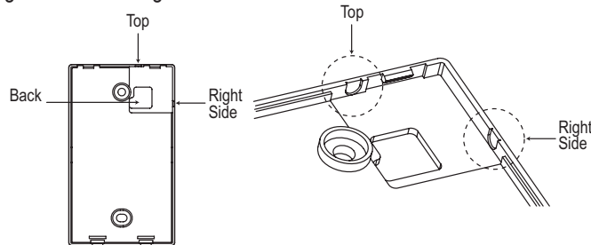
Figure 65:Installing/Removing the Controller.
