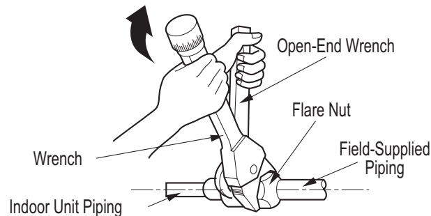
Figure 281: Using the Torque Wrench.
