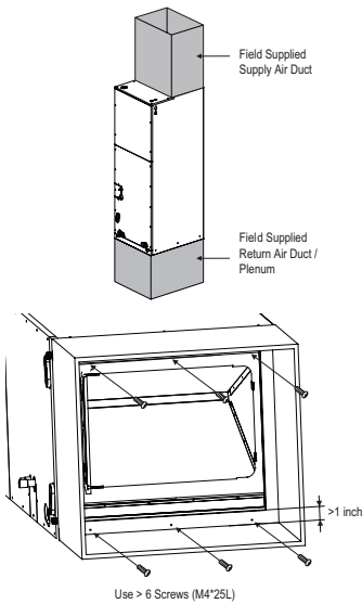
Figure 219:Vertical Installation / Attaching the Bottom Duct.
