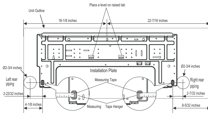
Figure 87: Installation Plate for LSN180HSV4 and LMN248HVT Units.
