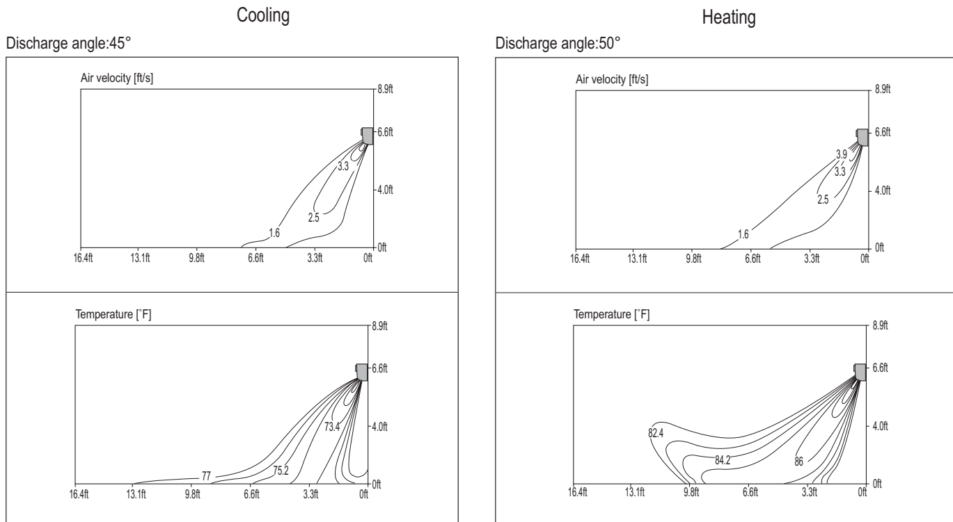
Figure 74:LSN090HSV4 Air Velocity and Temperature Distribution Charts.
