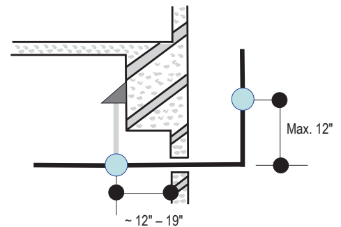
Figure 259: Typical Pipe Support Location—Change in Pipe Direction.
