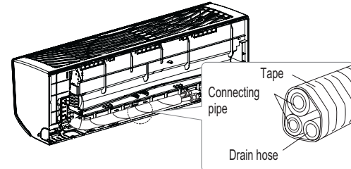
Figure 93: Piping Installed to the Left.
