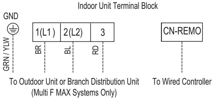
Figure 105:Wired Controller Connection on Indoor Unit Terminal Block—LMN078HVT, LSN090HSV4, LSN120HSV4, and LMN158HVT Models.
