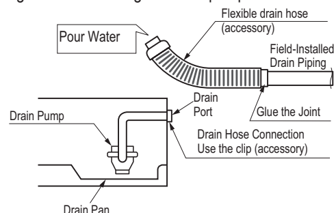
Figure 160: Checking the drain pump.
