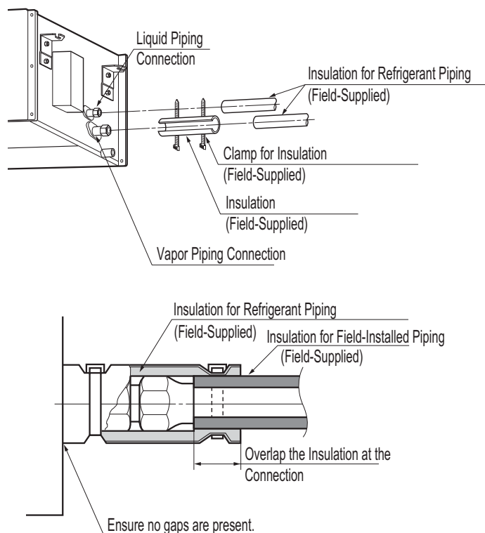
Figure 162: Insulating the Piping.
