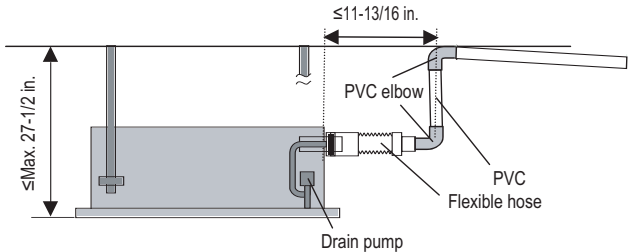
Figure 283:Diagram of an Indoor Unit with a Drain Pump.
