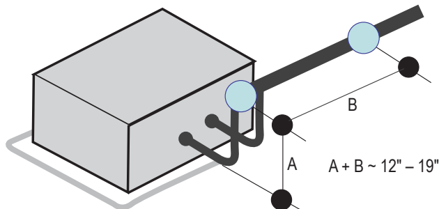
Figure 260: Pipe Support at Indoor Unit.
