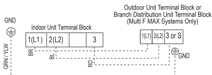
Figure 102: Simplified View of Indoor Unit to Outdoor Unit / Branch Distribution Unit Terminal Connections— LSN180HSV4 and LMN248HVT.
