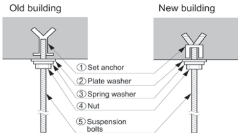
Figure 126:Console Bolt Options.
