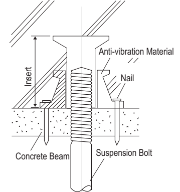
Figure 258: Pipe Hanger Details.
