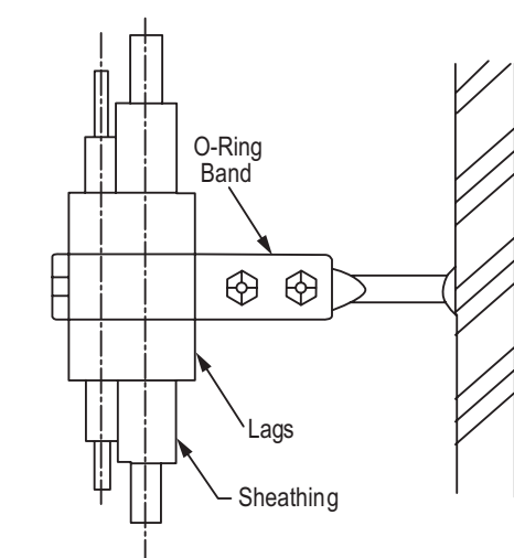
Figure 266:O-Ring Band Support with an Insulated Pipe.
