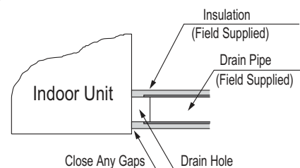
Figure 128: Drain Connection.
