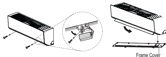
Figure 91: Removing the Frame Cover.
