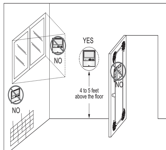
Figure 142: Proper Location for the Wired Controller.
