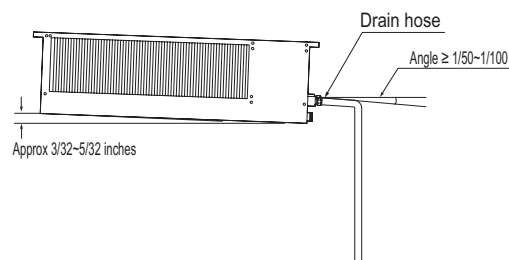
Figure 131: Checking the Drain Pump.
