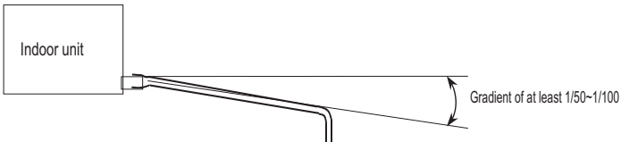
Figure 285:Drain Piping Gradient Recommendation.
