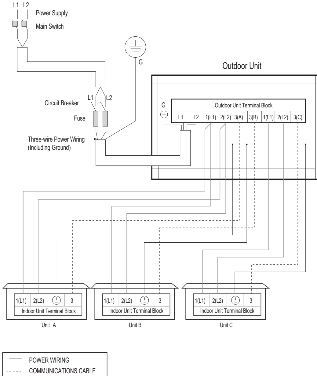
Figure 300: Multi F LMU24CHV System Power Wiring and Communications Cable.
