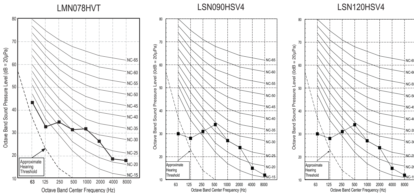
Figure 71: LMN078HVT, LSN090HSV4, and LSN120HSV4 Sound Pressure Level Diagrams.
