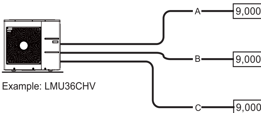
Figure 253: Multi F Additional Refrigerant Charge Example.
