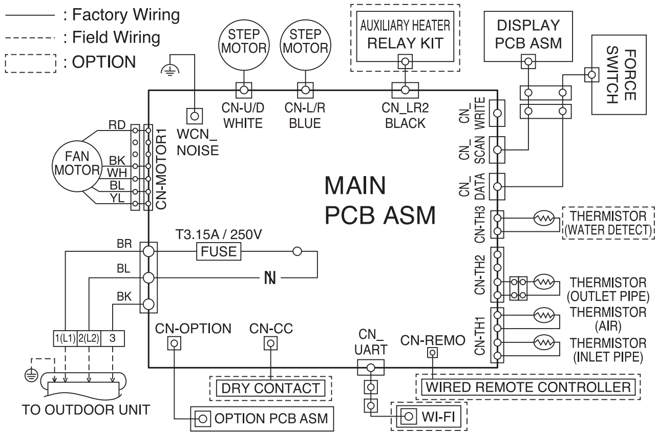
Figure 80: Multi F Standard Wall-Mounted LMN078HVT and LMN158HVT Indoor Units Wiring Diagram.
