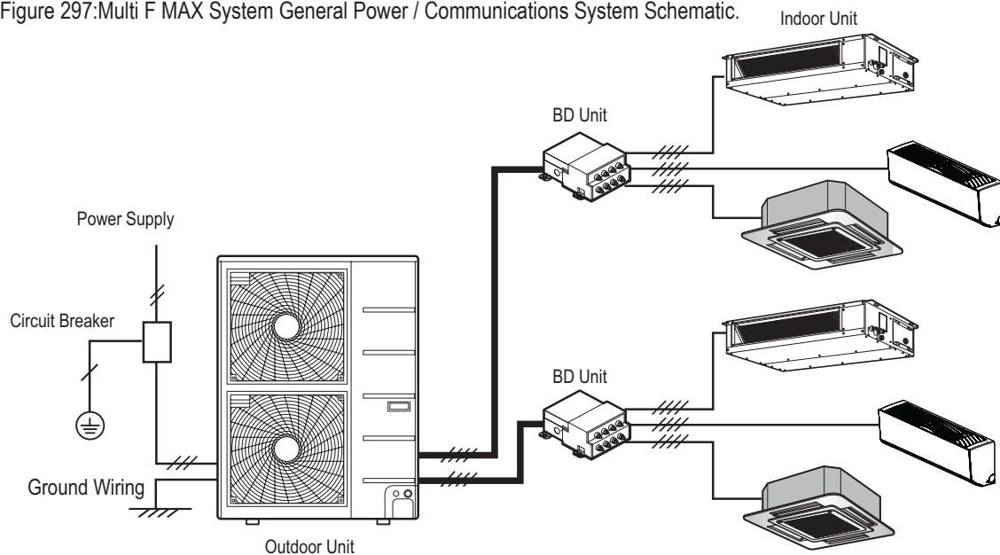
Figure 297: Multi F MAX System General Power / Communications System Schematic.
