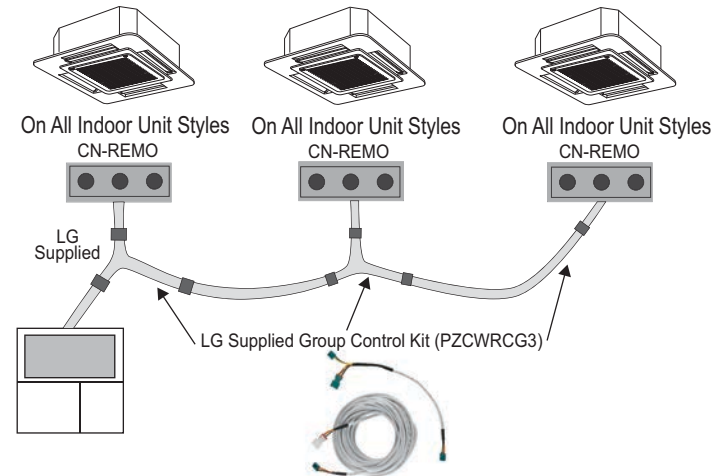
Figure 303:Indoor Unit Group to Zone Controller Connections.
