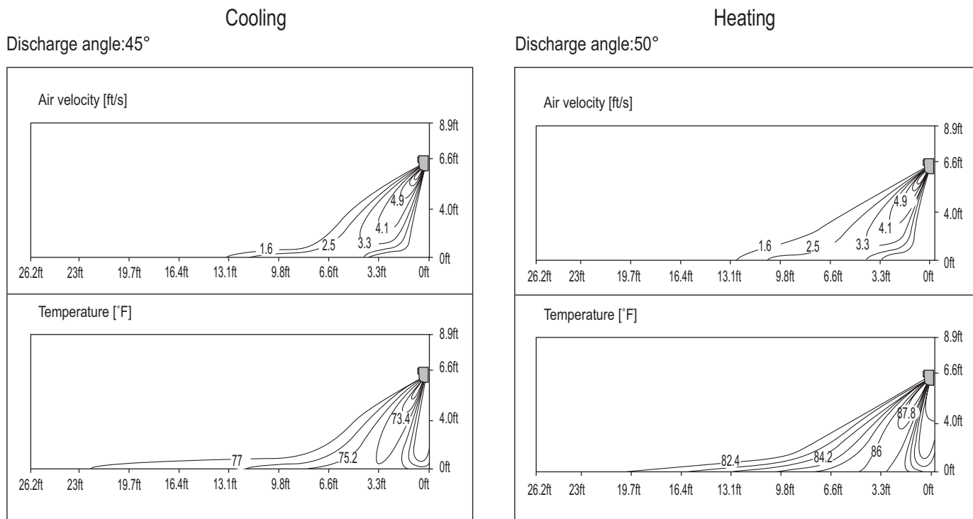
Figure 77: LSN180HSV4 Air Velocity and Temperature Distribution Charts.
