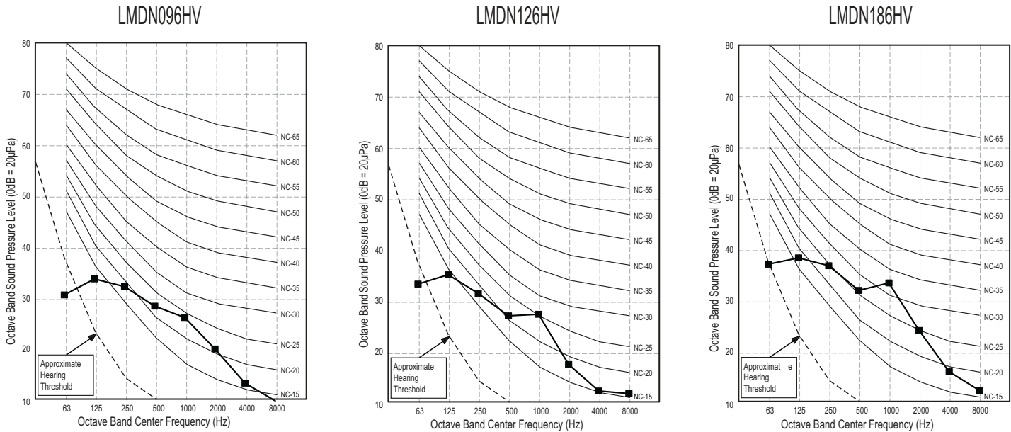
Figure 116: Sound Pressure Level Diagrams.
