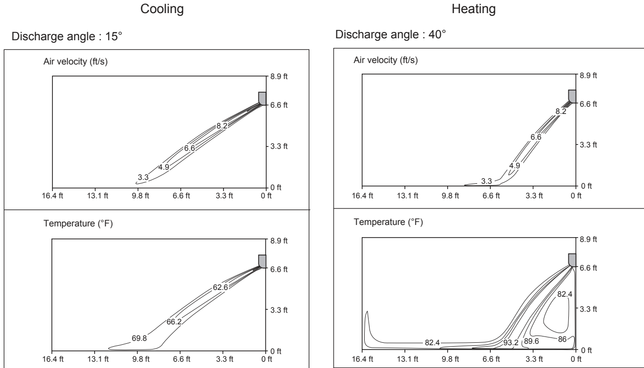
Figure 73:LMN078HVT Air Velocity and Temperature Distribution Charts.
