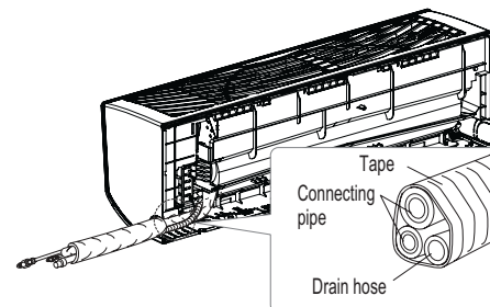
Figure 94: Piping Installed to the Right.
