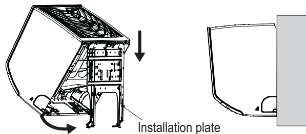
Figure 89: Locking the Indoor Unit onto the Installation Plate.
