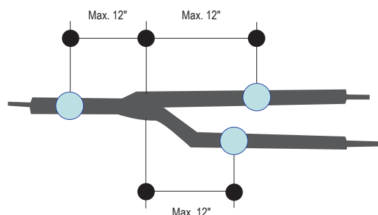
Figure 261: Pipe Support at Y-branch Fitting.
