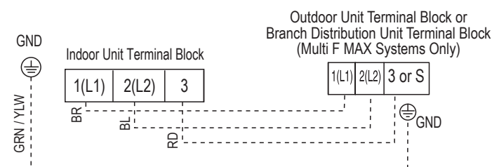
Figure 59: Simplified View of Indoor Unit to Outdoor Unit / Branch Distribution Unit Terminal Connections—LMAN097HVP and LMAN127HVP models.
