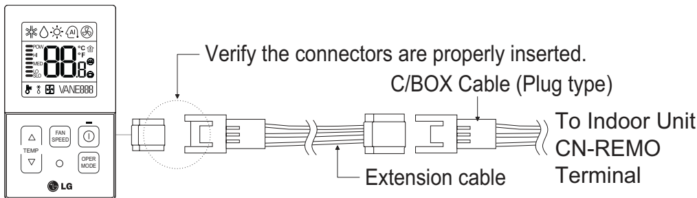
Figure 232:PZCWRC1 LG Wired Remote Extension Cable.
