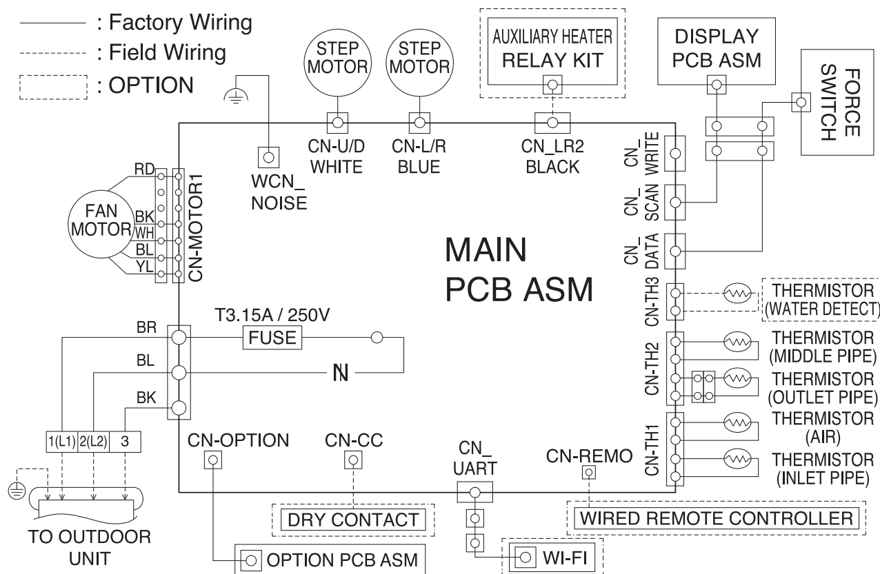
Figure 82:Multi F Standard Wall-Mounted LSN090HSV4 and LSN120HSV4 Indoor Units Wiring Diagram.
