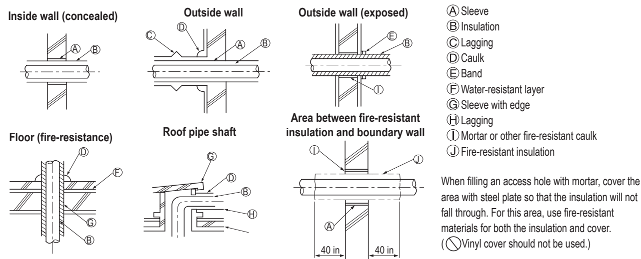
Figure 269:Pipe Sleeve Options.
