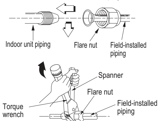
Figure 53: Indoor Unit to Field-Installed Piping Connection.
