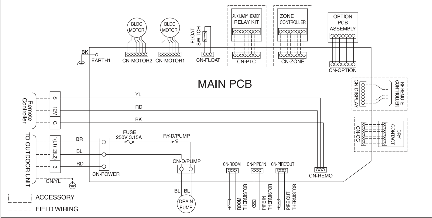
Figure 119:Multi F Ceiling-Concealed Duct (Low Static) LMDN096HV, LMDN126HV, and LMDN186HV Indoor Units Wiring Diagram.
