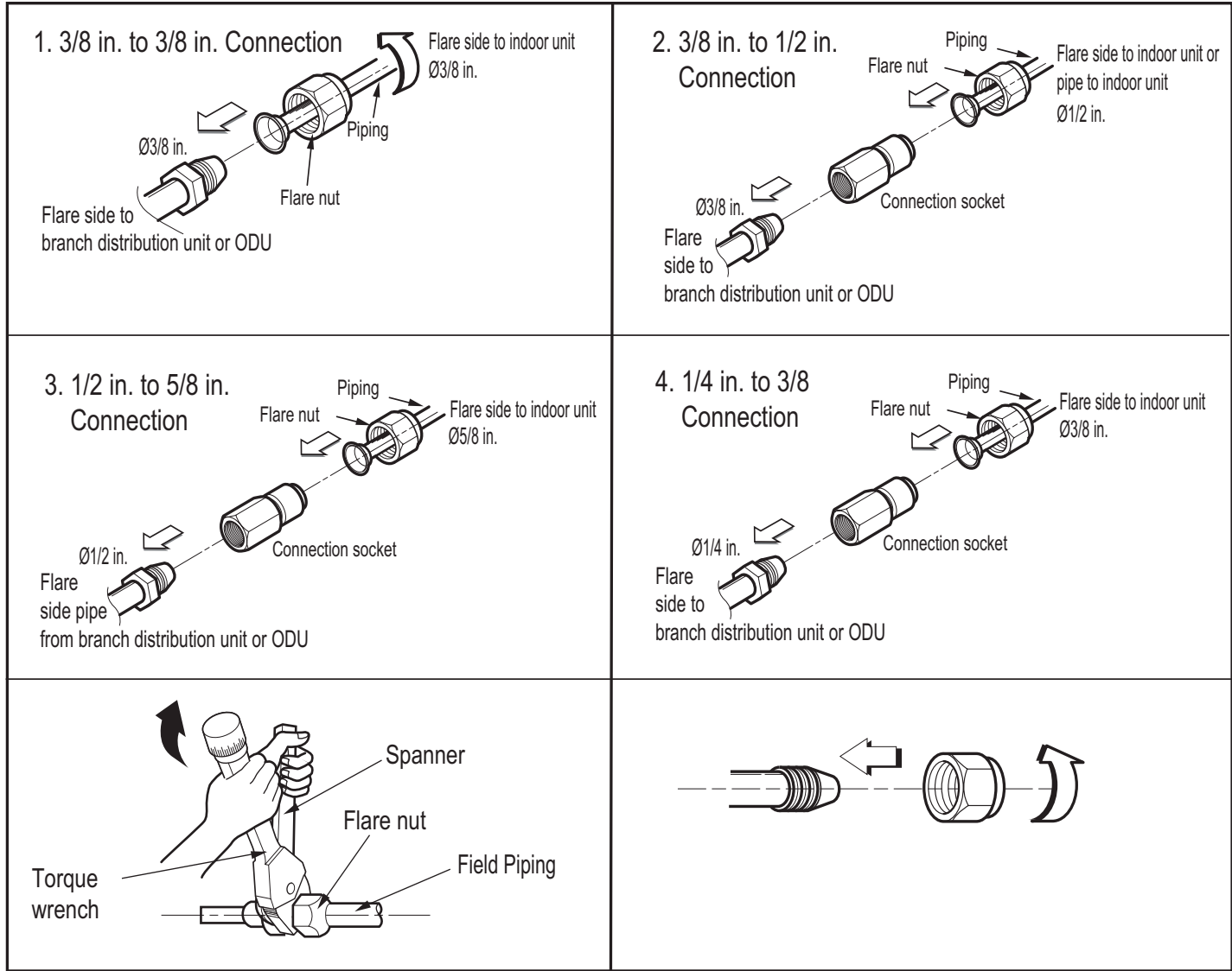
Figure 277: Possible Outdoor Unit or Branch Distribution Unit to Indoor Unit Connections.
