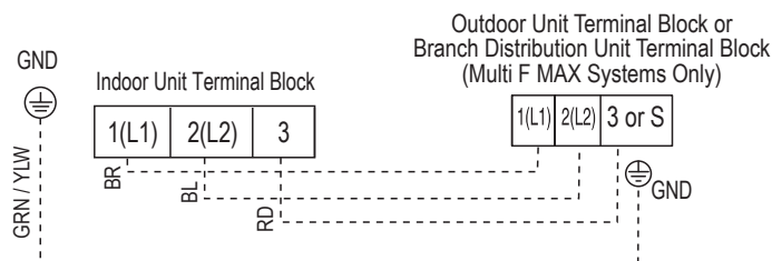
Figure 101: Simplified View of Indoor Unit to Outdoor Unit / Branch Distribution Unit Terminal Connections—LMN078HVT, LSN090HSV4, LSN120HSV4 and LMN158HVT.
