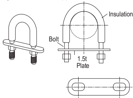
Figure 262:U-Bolt Support with Insulation.
