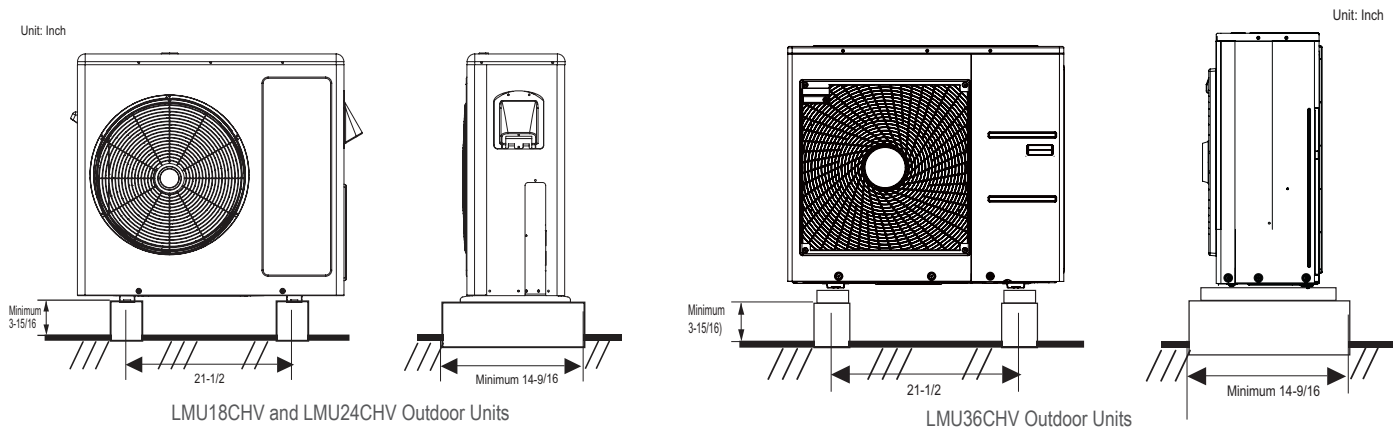
Figure 244: Outdoor Unit Foundation Requirements.
