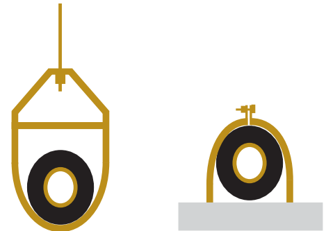
Figure 259: Typical Pipe Support Location—Change in Pipe Direction.
