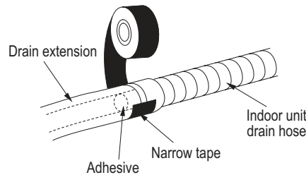
Figure 96: Extending the Drain Hose.
