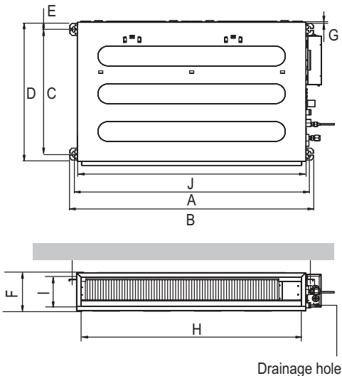
Figure 124: Indoor Unit Bolt Locations.
