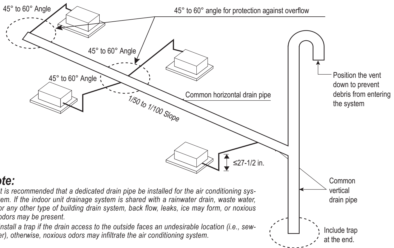
Figure 286: Example of a Common Indoor Unit Drainage System.
