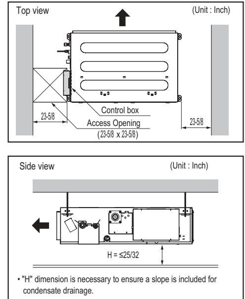
Figure 120: General Installation Guidelines.
