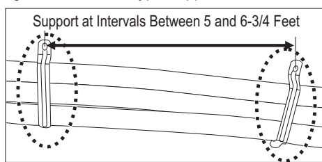
Figure 264:Saddle-Type Support.
