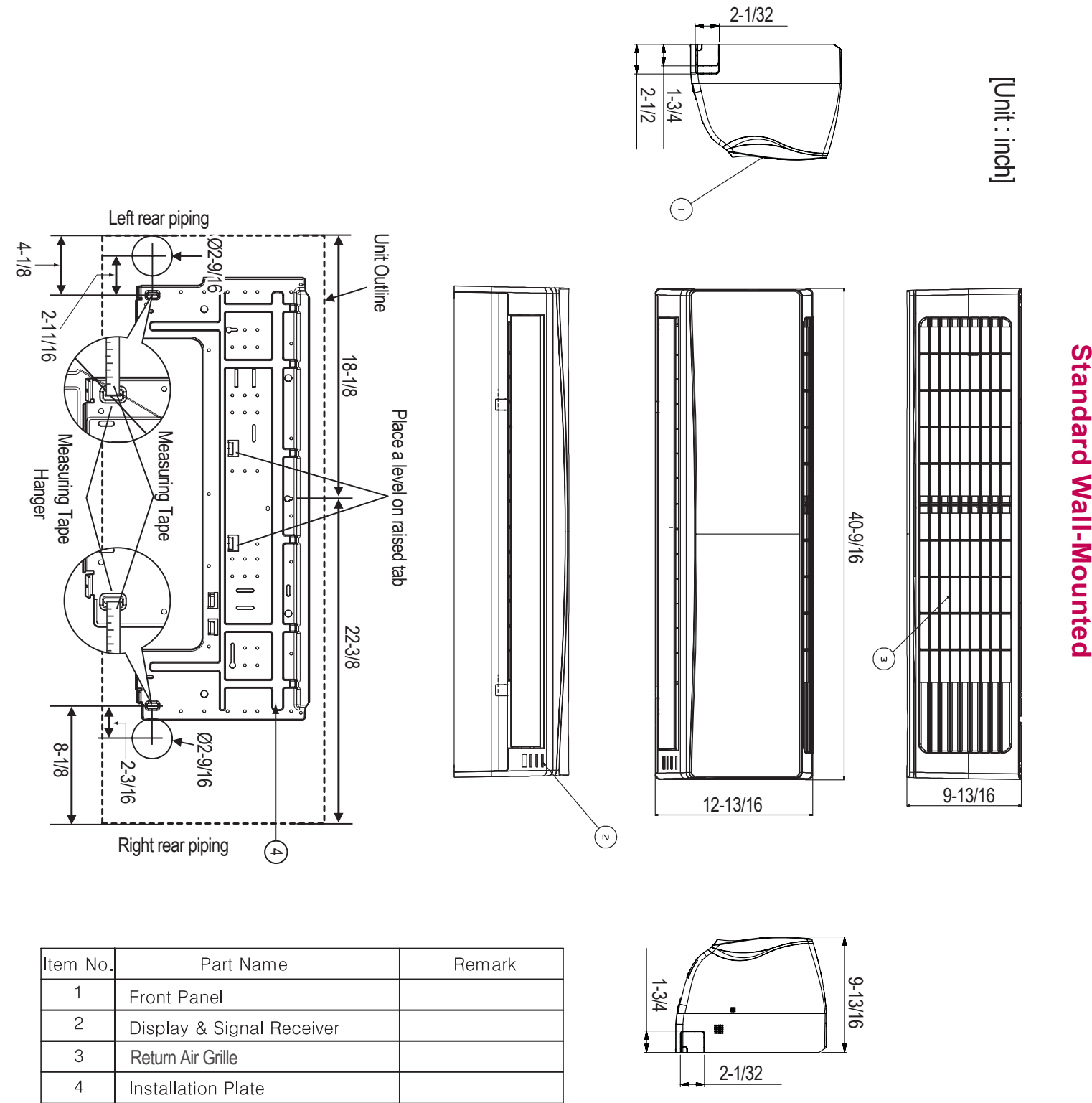
Figure 69: LSN180HSV4 and LMN248HVT Dimensions.
