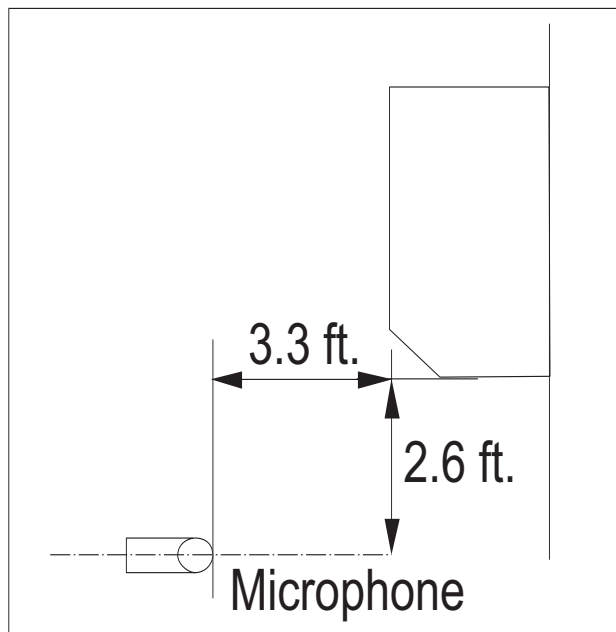
Figure 70: Sound Pressure Level Measurement Location.
