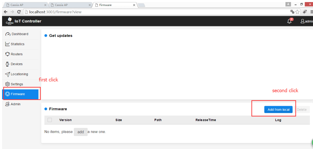
Figure 10: Upload firmware to AC
