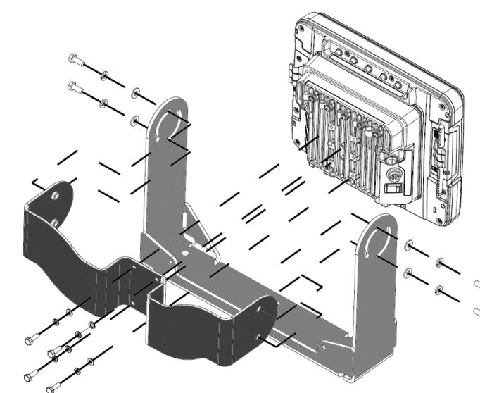
Exploded View of adapter plate installed into U-Bracket.
