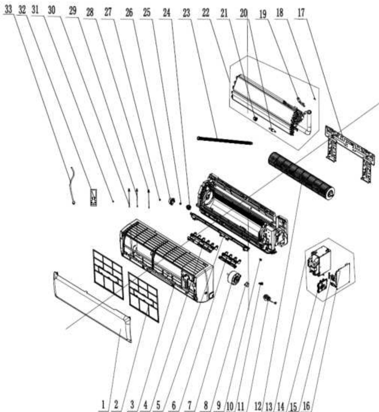
Exploded View of GMV-ND45G/B6B-T、GMV-ND50G/B6B-T:
