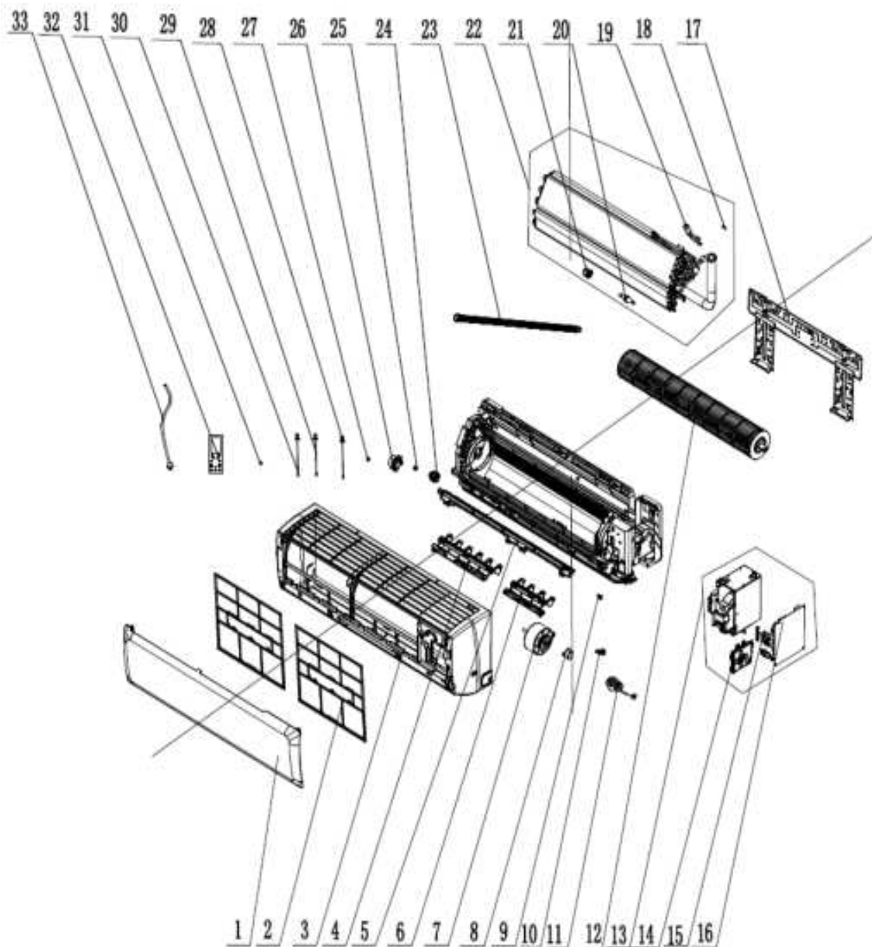
Exploded View of GMV-ND56G/B6B-T、GMV-ND63G/B6B-T、GMV-ND71G/B6B-T:
