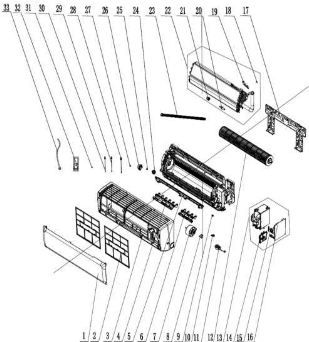
Exploded View of GMV-ND22G/C4B-T、GMV-ND28G/C4B-T、GMV-ND36G/C4B-T:
