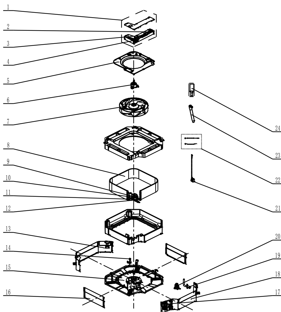
Exploded View of GMV-ND22T/C1-T,GMV-ND28T/C1-T,GMV-ND36T/C1-T:
