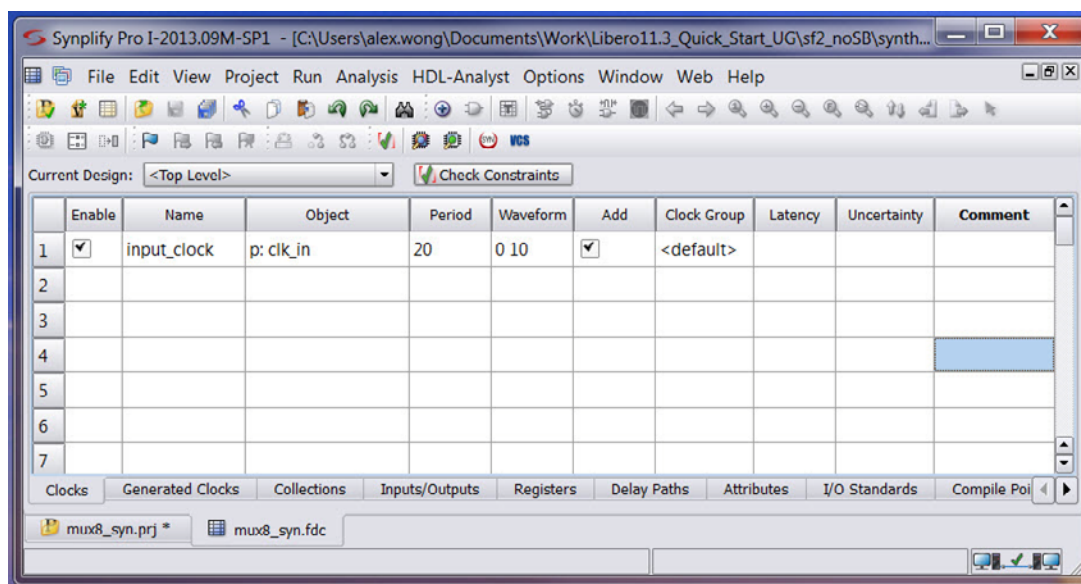
Figure 2-4 • Clocks Tab
