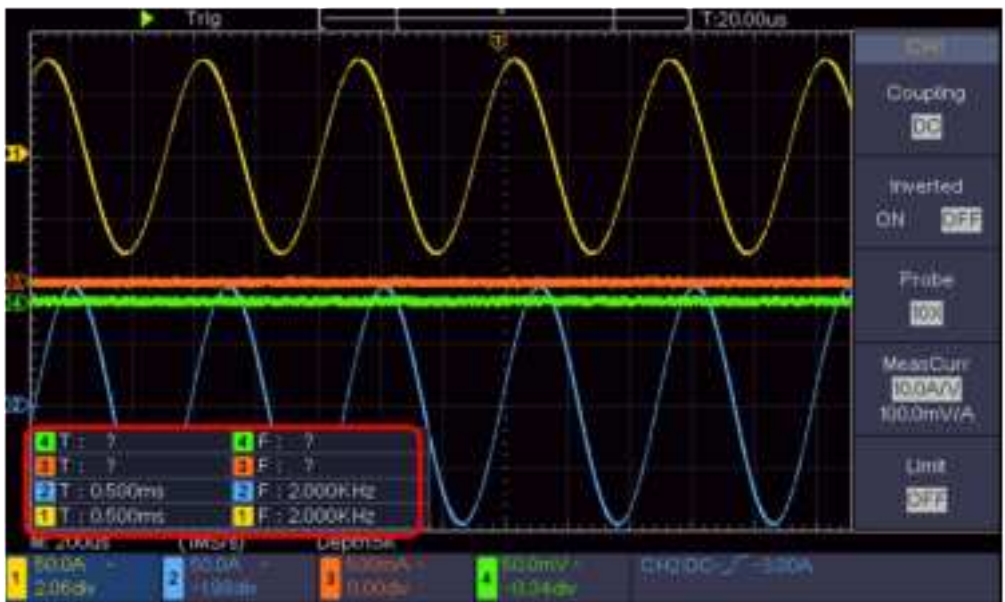
Figure 4- 12 Automatic measurement
