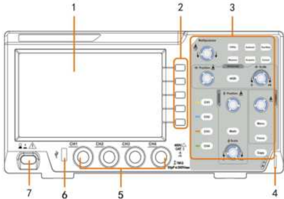
Figure 3- 1 Front panel
