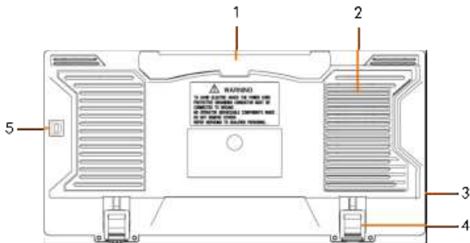
Figure 3-2 Rear Panel
