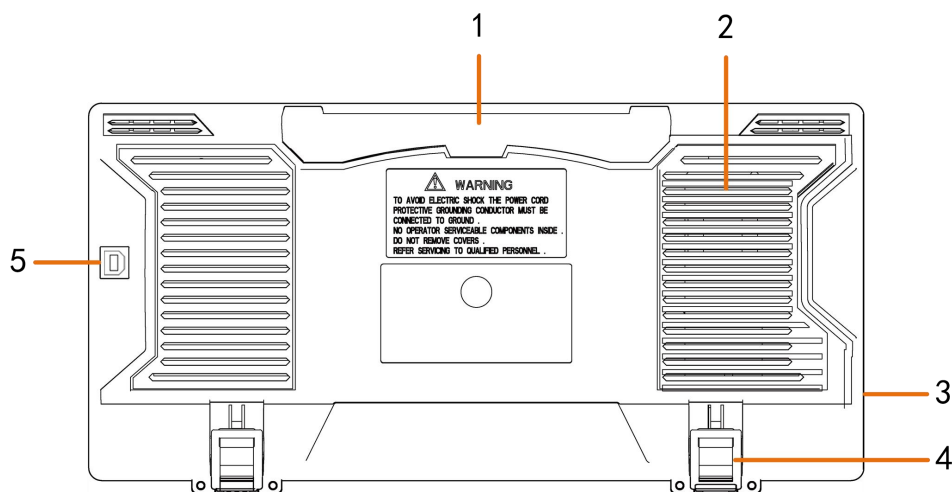
Figure 3-2 Rear Panel
