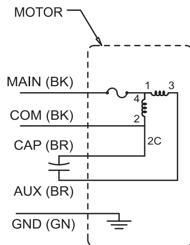
SCHEMATIC
