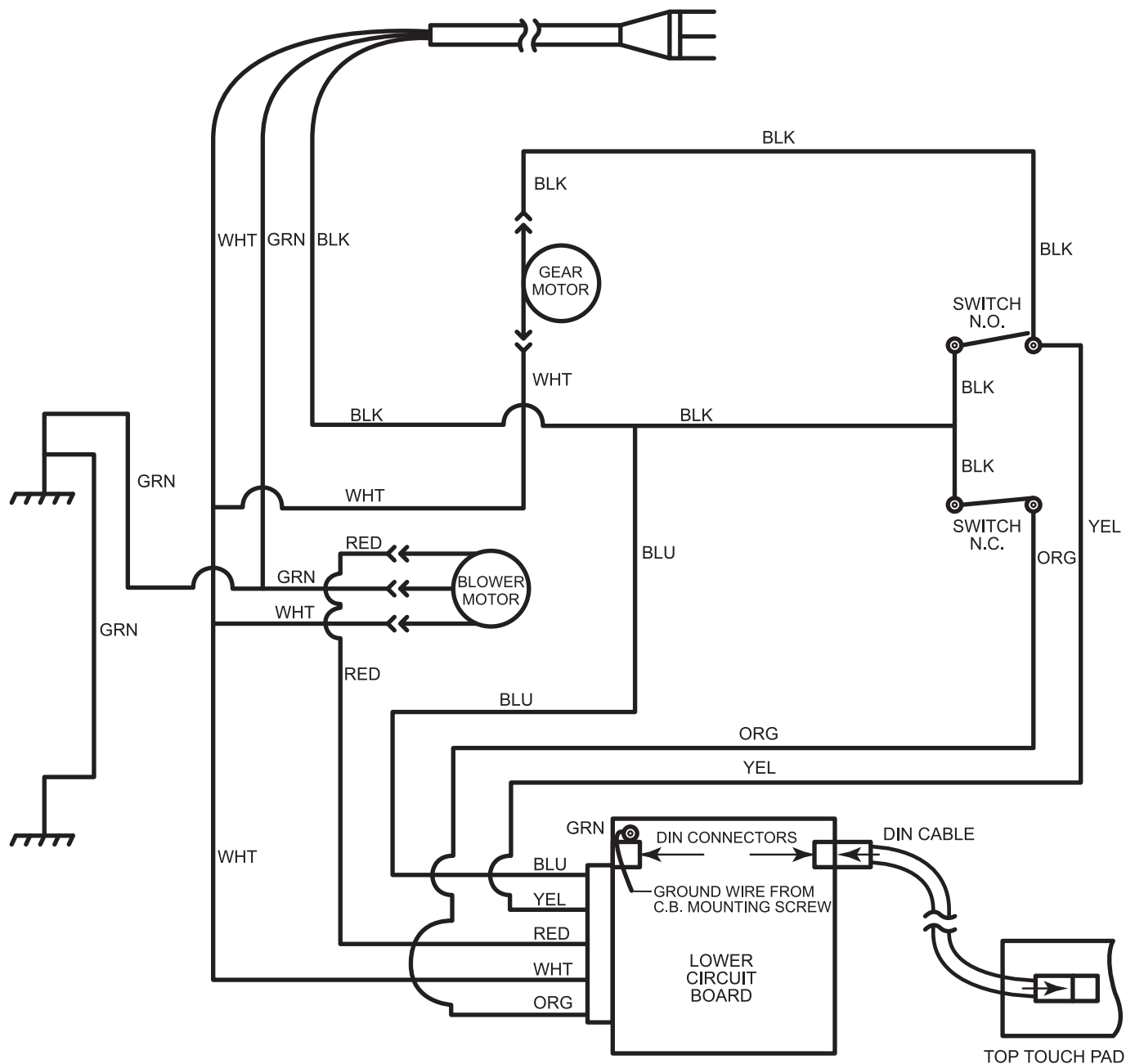
DOWNDRAFT WIRING DIAGRAM
