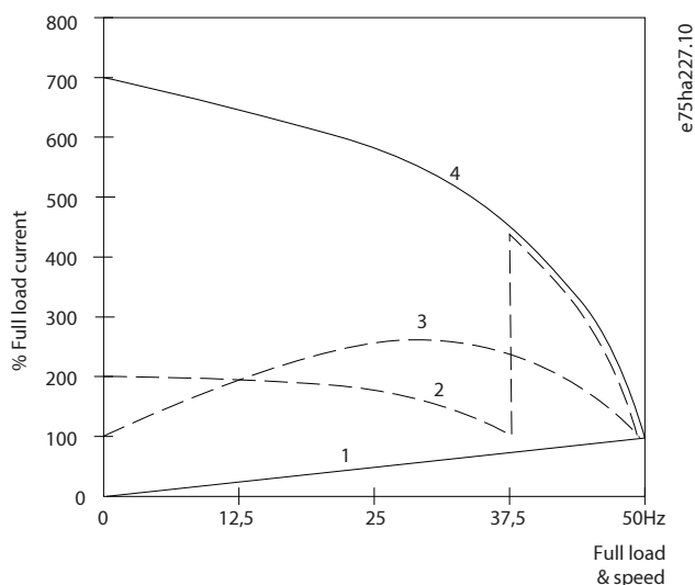
Figure 15: Start-up Current
