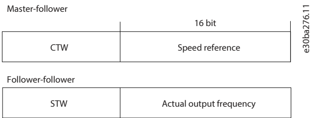
Figure 117: Actual Output Frequency (MAV)
