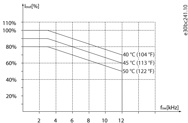
Figure 45: 37 kW (50 hp), 400 V, Enclosure Size I6, IP54
