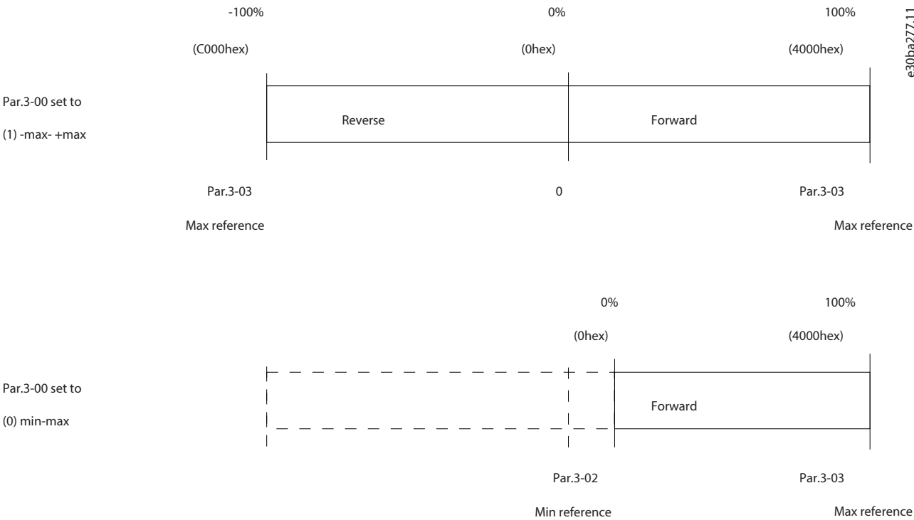
Figure 118: Reference and MAV
