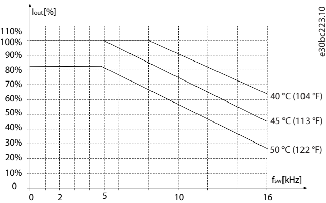
Figure 24: 5.5–7.5 kW (7.5–10 hp), 200 V, Enclosure Size H4, IP20/Open type
