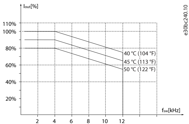
Figure 44: 22-30 kW (30-40 hp), 400 V, Enclosure Size I6, IP54
