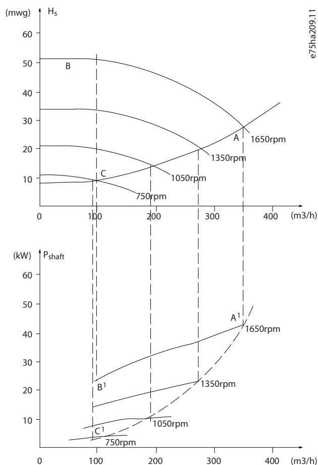
Figure 14: Energy
