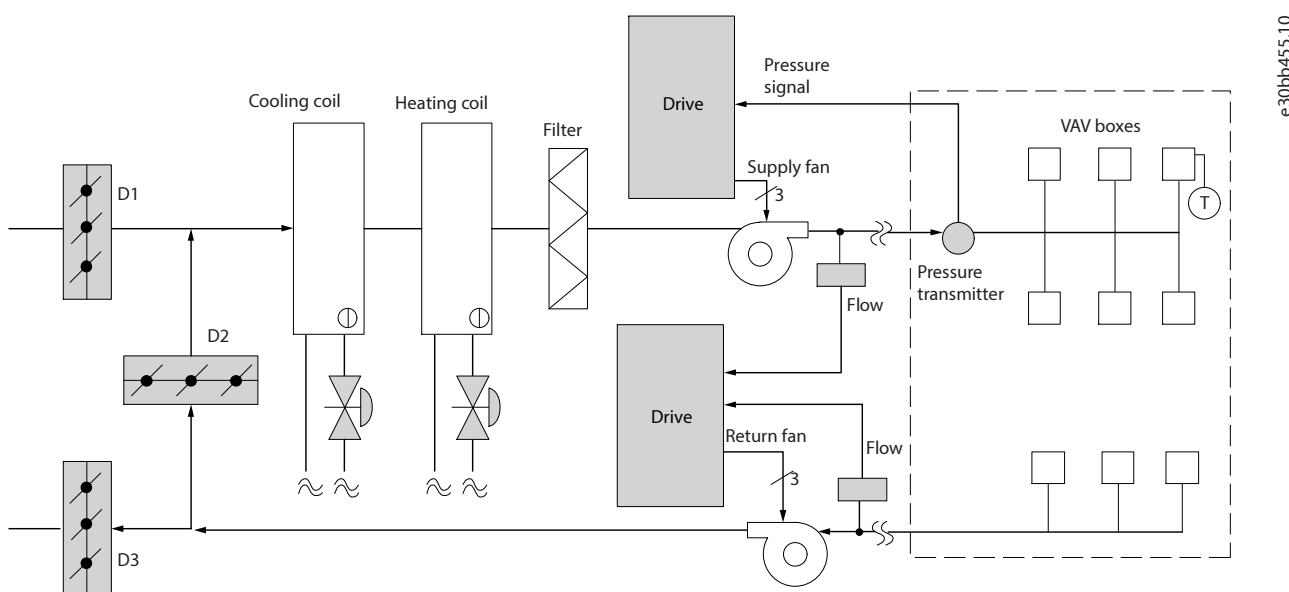
Figure 94: Variable Air Volume
