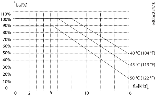
Figure 25: 11–15 kW (15–20 hp), 400 V, Enclosure Size H4, IP20/Open type
