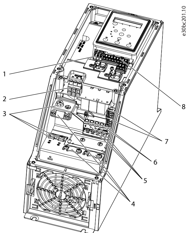
Figure 62: Enclosure Size I3, IP54, 380–480 V, 5.5–7.5 kW (7.5–10 hp)
