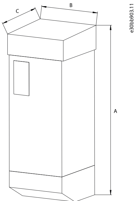
Figure 125: Dimensions
