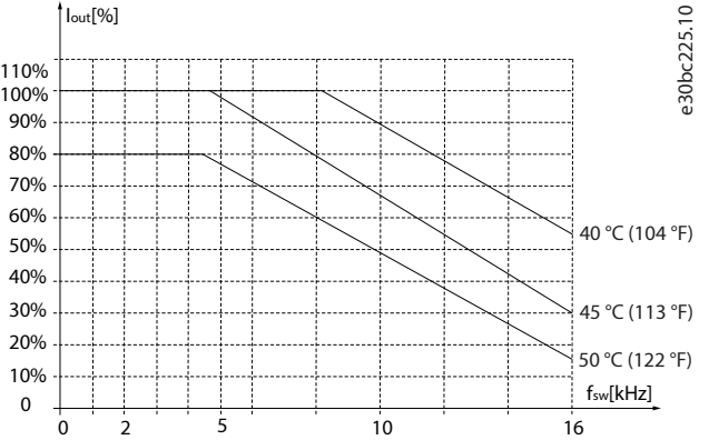
Figure 26: 11 kW (15 hp), 200 V, Enclosure Size H5, IP20/Open type
