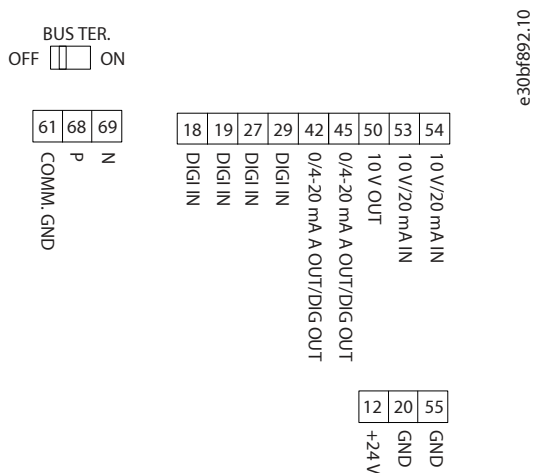
Figure 83: Control Terminals
