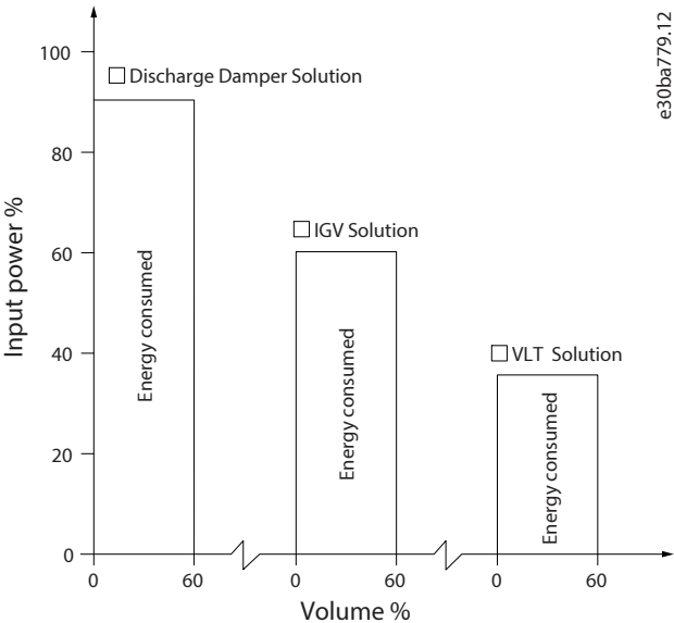
Figure 12: Energy Savings
