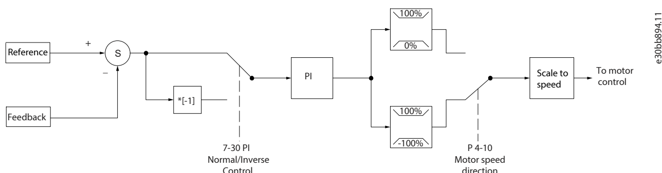
Figure 91: Control Structure Closed Loop
