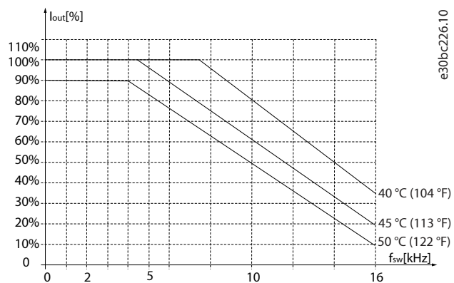
Figure 27: 18.5–22 kW (25–30 hp), 400 V, Enclosure Size H5, IP20/Open type
