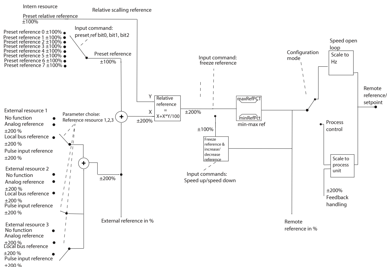
Figure 93: Block Diagram Showing Remote Reference
