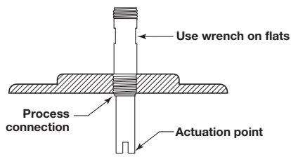
Figure 3 Vertical Mounting
