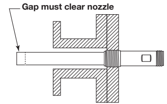
Figure 5 Nozzle Mounting
