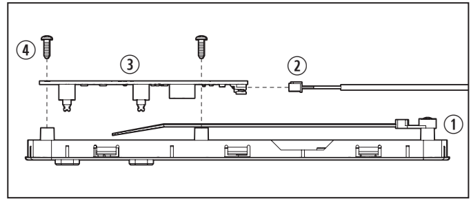
2 Removing the Circuit Board
