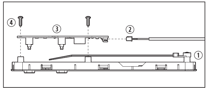
2 Removing the Circuit Board
