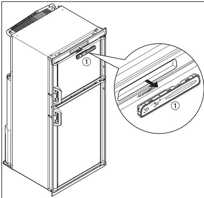
1 Removing the Control Interface Display
