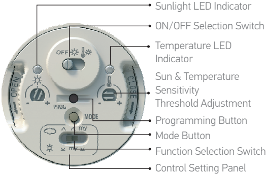
Front view with cover removed
