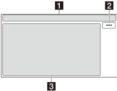
HOME screen:
