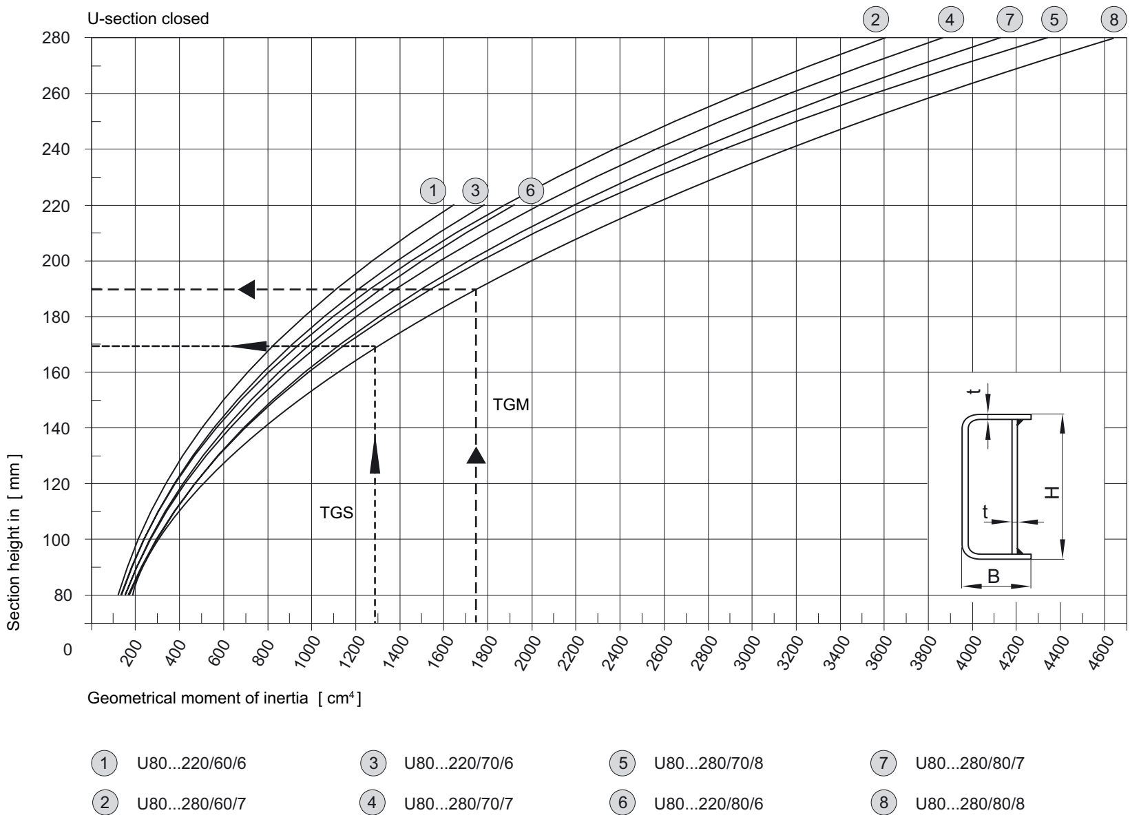
Fig. 108: Geometrical moment of inertia for open U-sections ESC-214
