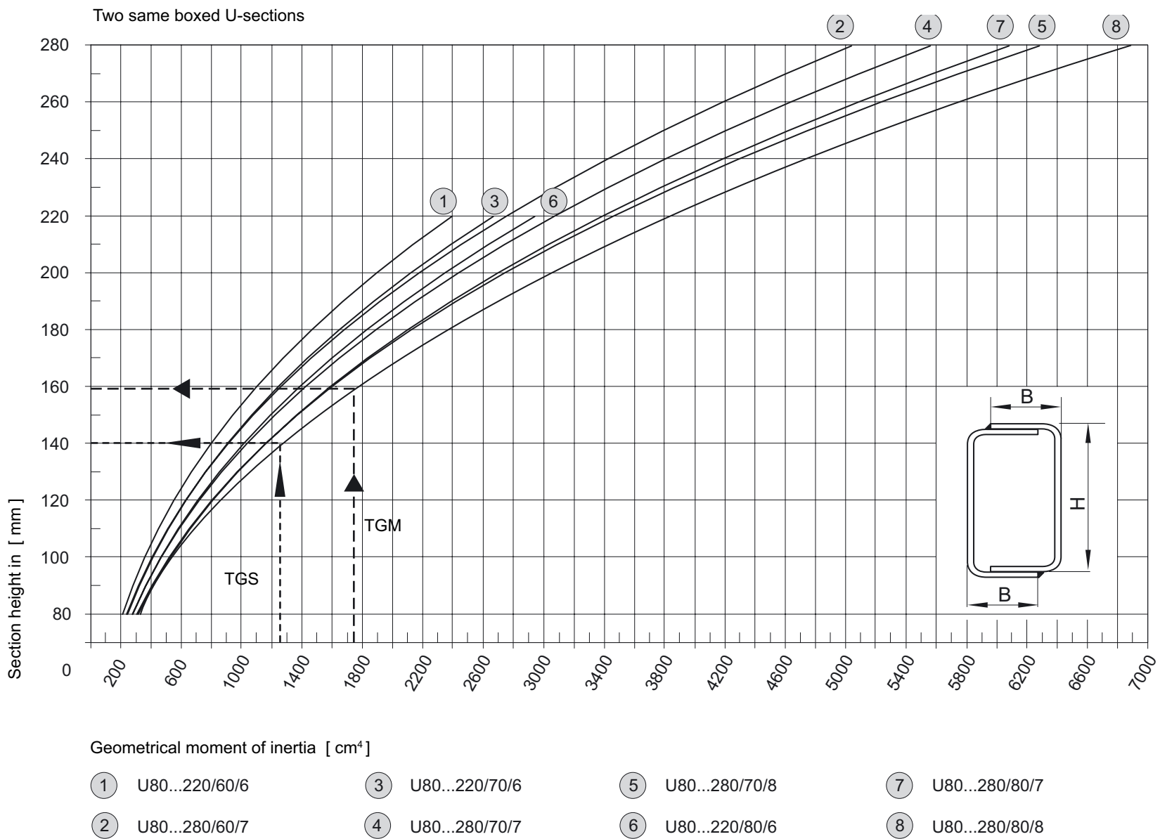
Fig. 109: Geometrical moment of inertia for boxed U-sections ESC-215
