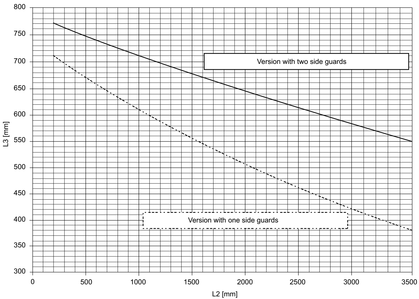
Fig. 44: Graph for ascertaining the span and projection ESC-220
