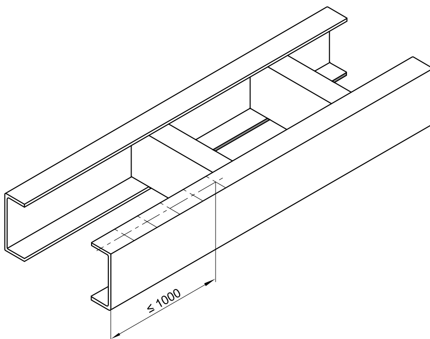
Fig. 11: Drill holes at frame end ESC-032
