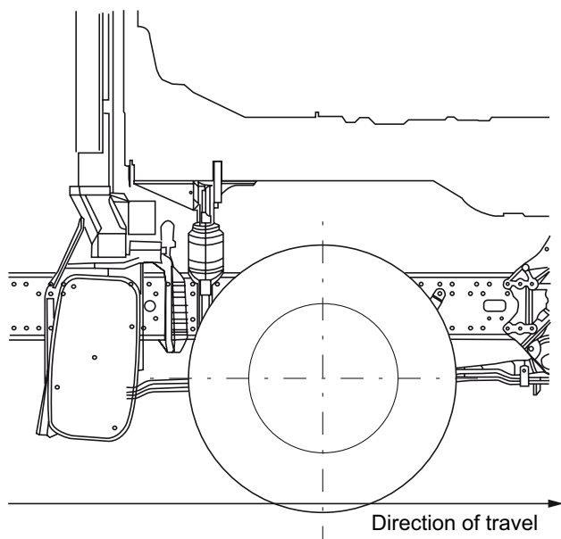
Fig. 60: L-XXL cab, raised exhaust endpipe ESC-729
