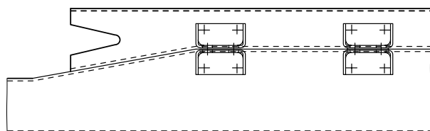
Fig.77: Subframe - adapting by widening ESC-098
