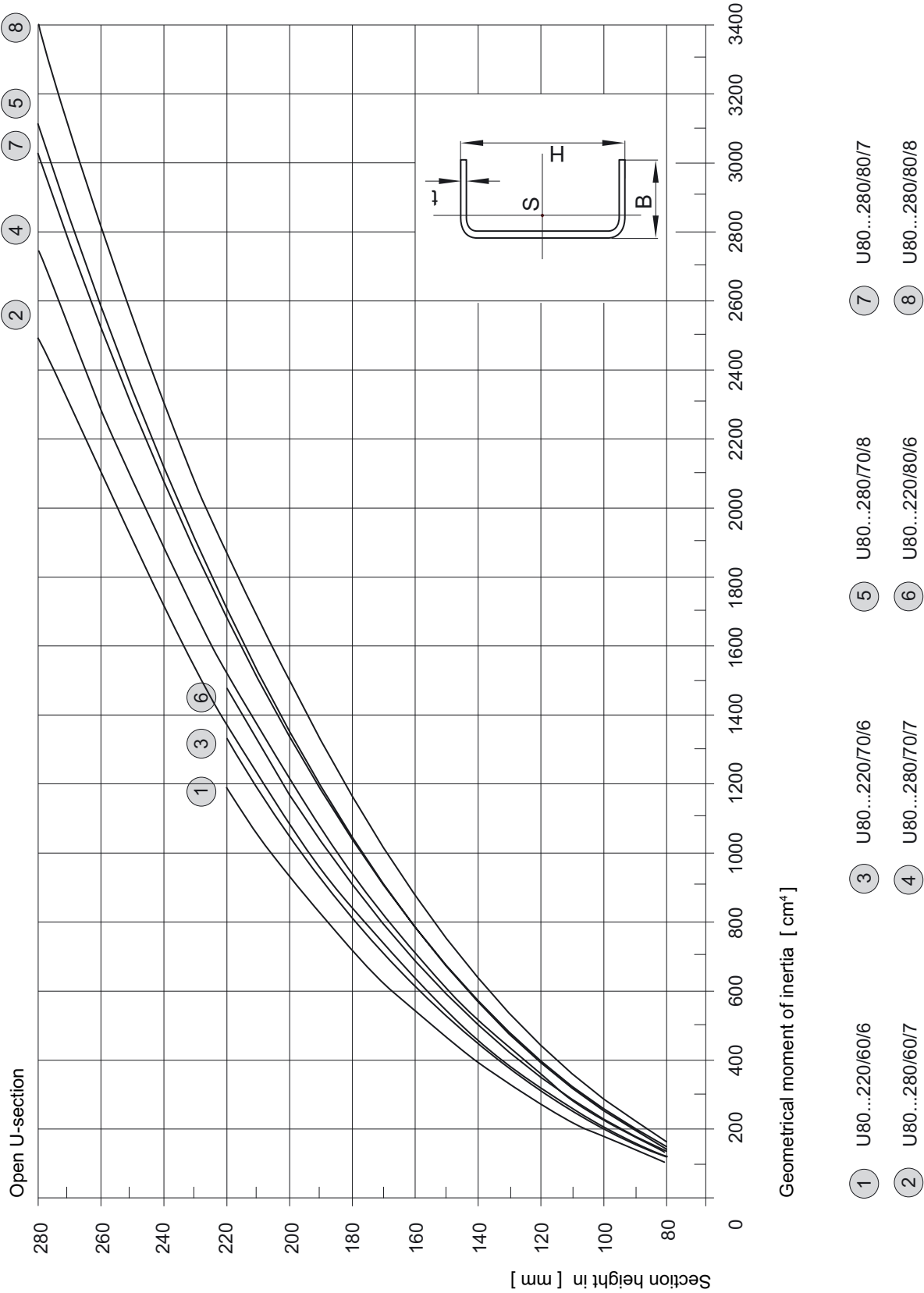
Fig. 107: Geometrical moment of inertia for U-sections ESC-213
