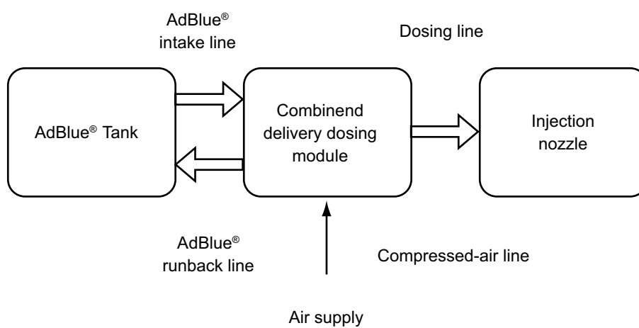
Fig. 68: Schematic overview of the AdBlue® system in Euro 6 vehicles ESC-419a
