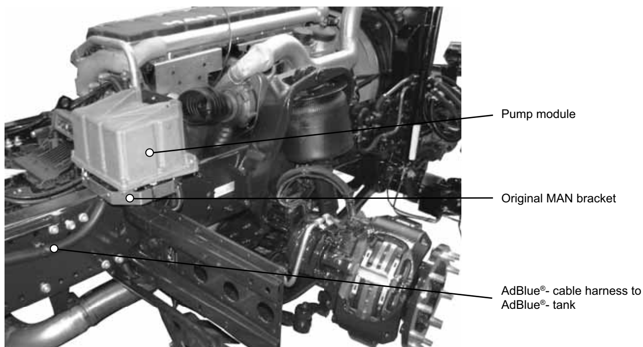
Fig. 50: Pump module and original MAN bracket ESC-421
