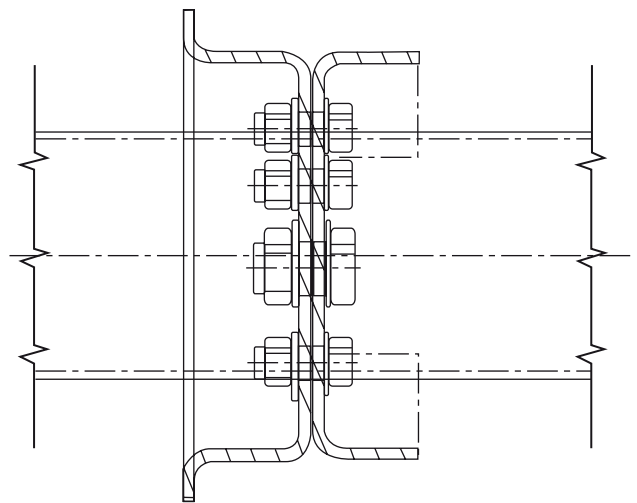
Fig.42: Lower bolted connection, underride guard bracket ESC-524
