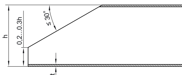
Fig. 75: Subframe taper at front ESC-030
