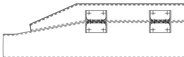
Fig. 78: Subframe - adapting by tapering ESC-099
