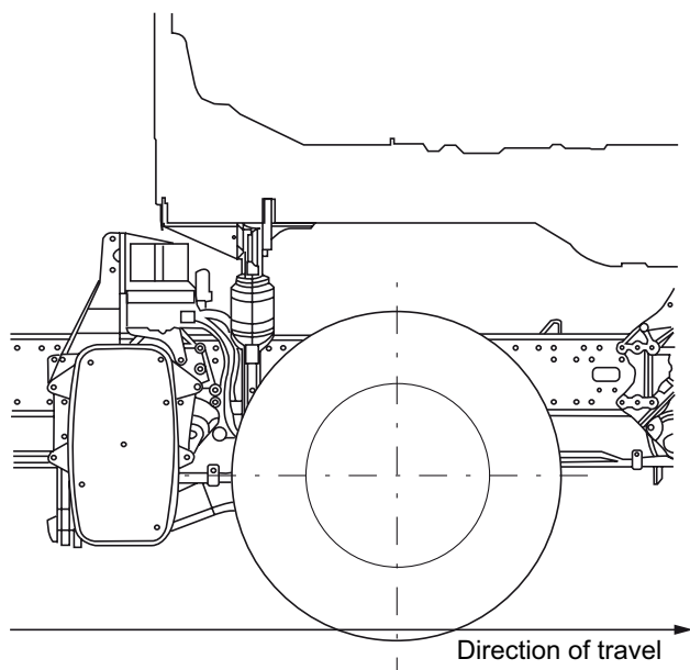
Fig. 61: L-LX cab, diagonally above the frame upper edge rotated through 180°, right-hand side mounted exhaust ESC-730
