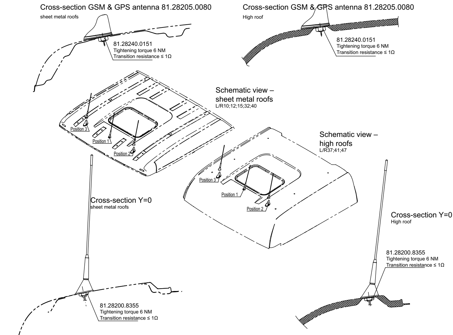
Fig. 112: Antenna installation positions ESC-560
