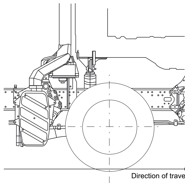
Fig. 59: Longitudinally above the frame, raised exhaust endpipe, M cab ESC-728
