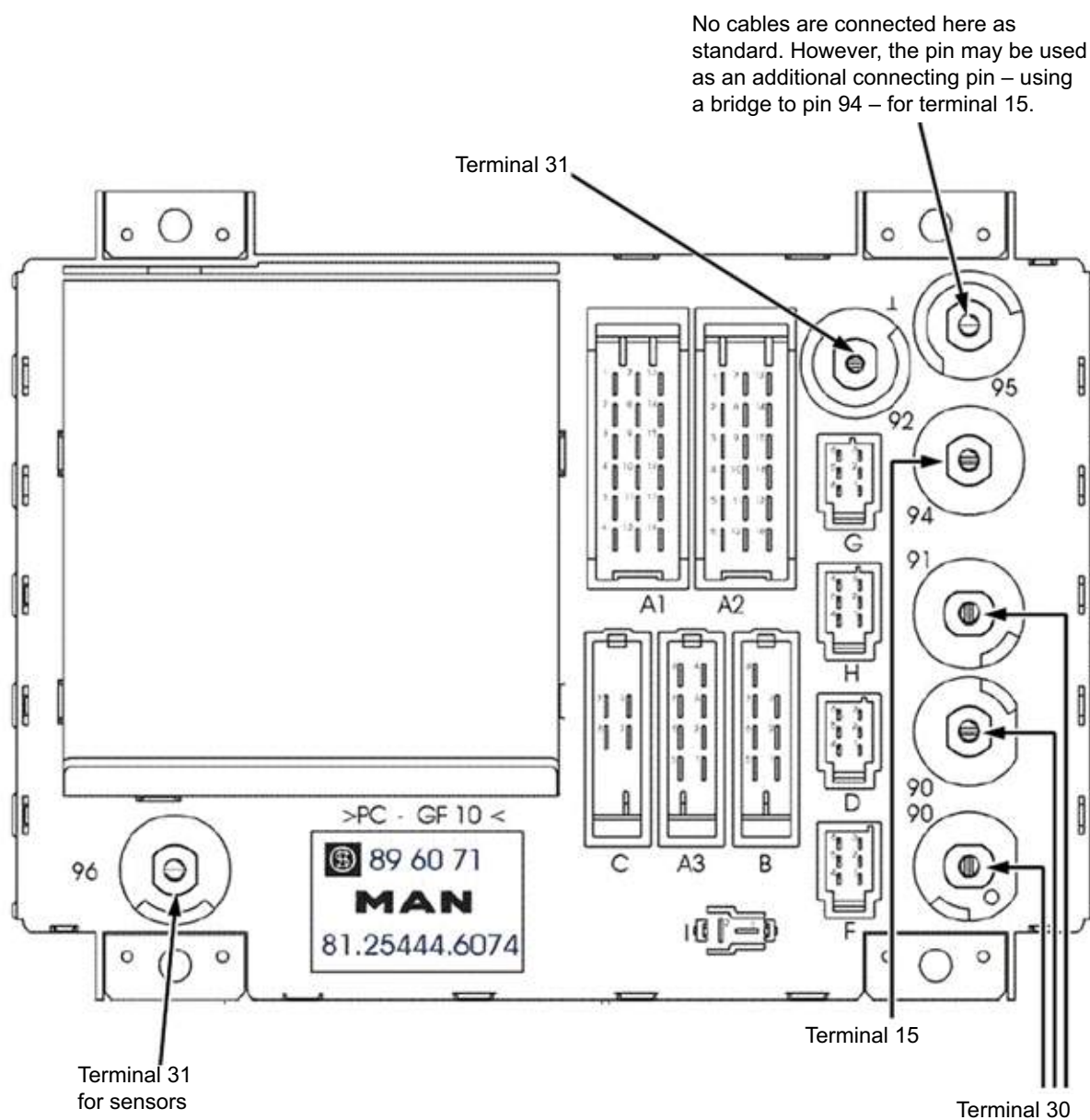
Fig. 111: Central electrics box, rear view ESC-720
