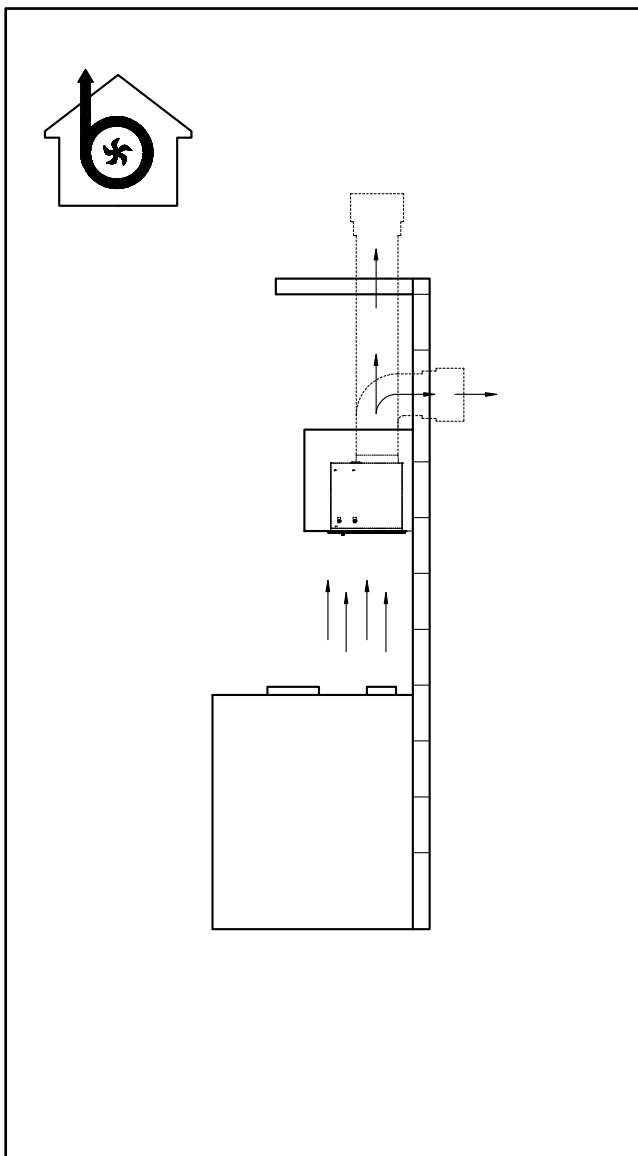
Extraction-air mode
