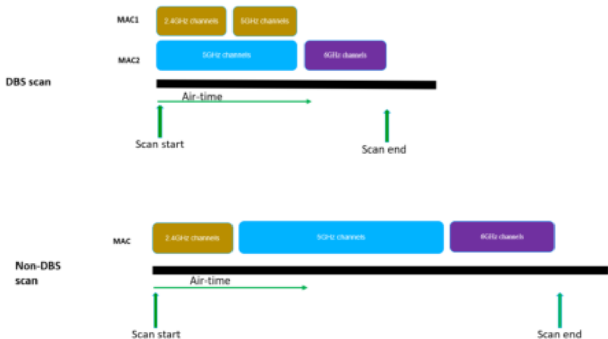
Figure 2 Wi-Fi Scanning
