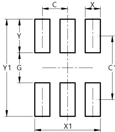
SOT563 (Standard)
