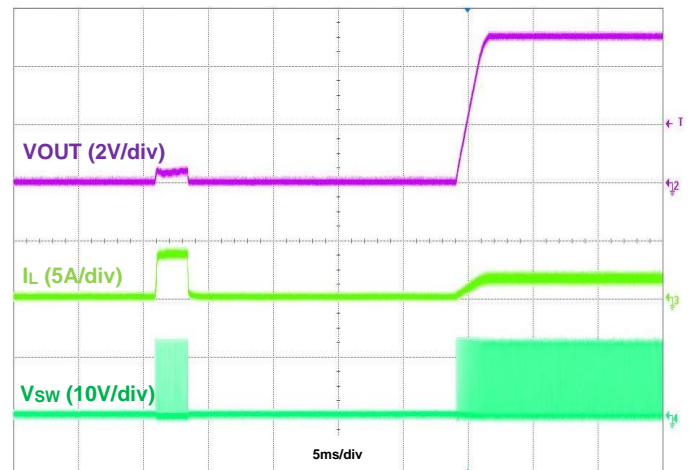
Figure 23. Output Short Recovery, I_{OUT} = 1.5\text{A}
