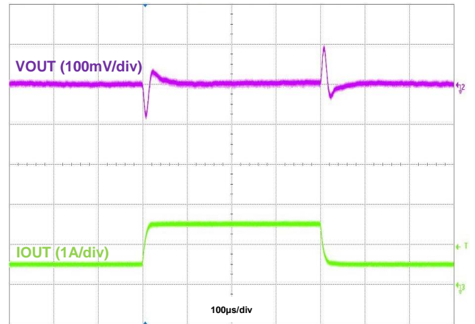
Figure 18. Load Transient, I_{OUT} = 0.5\text{A} to 1.5\text{A} to 0.5\text{A}
