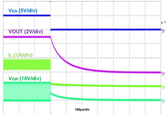
Figure 21. Shutdown Using EN, I_{OUT} = 1.5\text{A}
