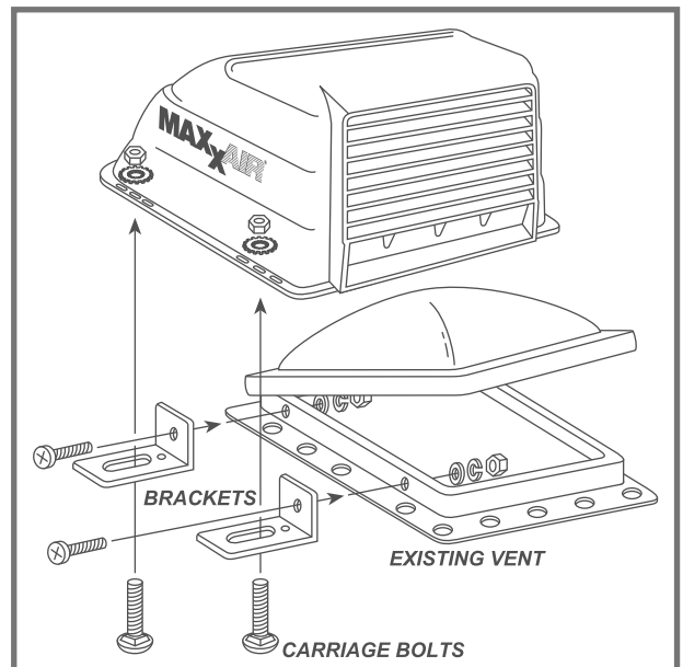
MAXXAIR VENT COVER
