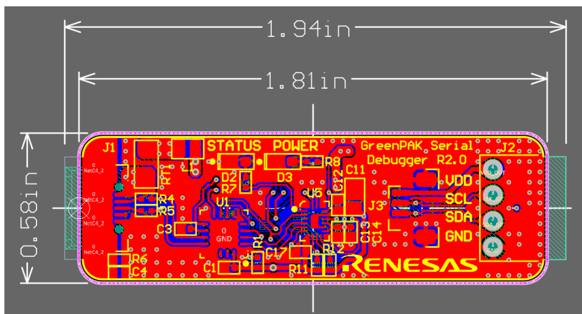
Figure 2: PCB
