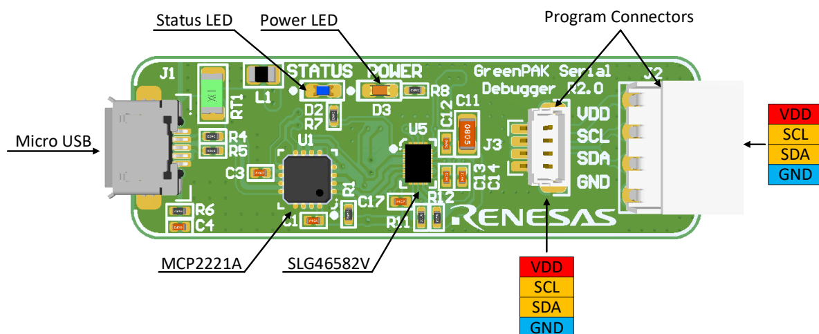
Figure 1: GreenPAK Serial Debugger Top View
