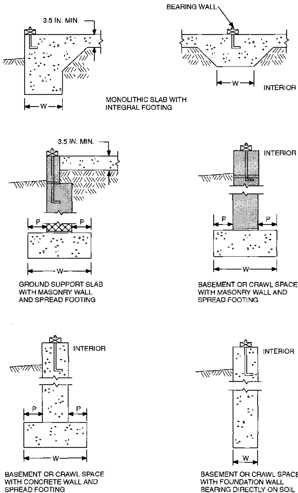
FIGURE R403.1(1) CONCRETE AND MASONRY FOUNDATION DETAILS
