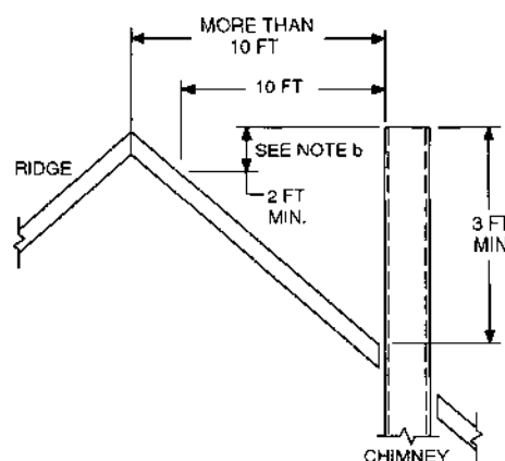
B. TERMINATION MORE THAN 10 FT FROM RIDGE, WALL OR PARAPET
