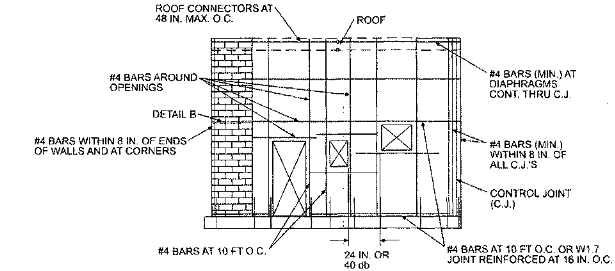
MINIMUM REINFORCEMENT FOR MASONRY WALLS
