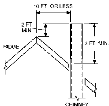
A. TERMINATION 10 FT OR LESS FROM RIDGE, WALL OR PARAPET
