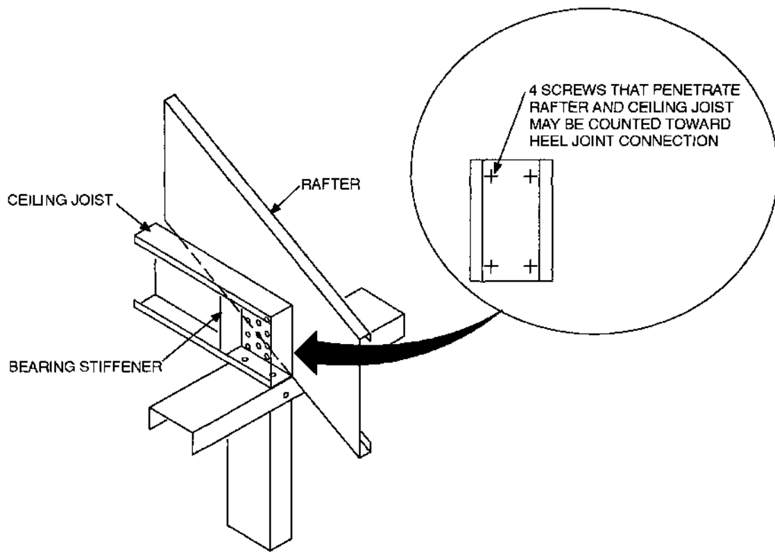
FIGURE R804.3.8 BEARING STIFFENER
