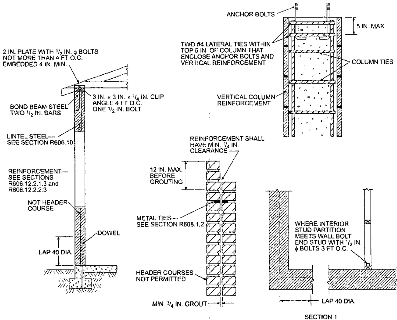
MINIMUM REINFORCEMENT FOR MASONRY WALLS
