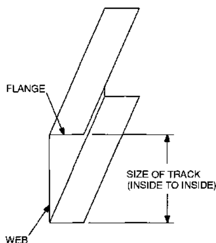
FIGURE R804.2(2) TRACK SECTION
