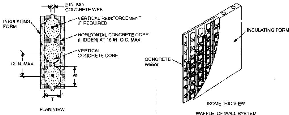
FIGURE R611.4 WAFFLE-GRID ICF WALL SYSTEM
