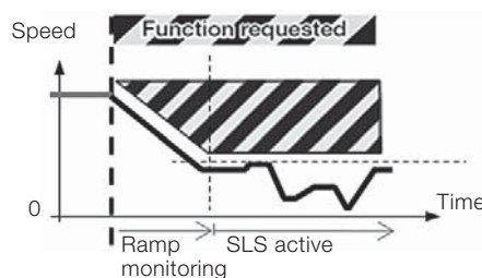
Figure 1: Safely-limited speed (SLS) function using the ramp monitoring method.
