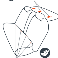
LATCH Lower Anchors
