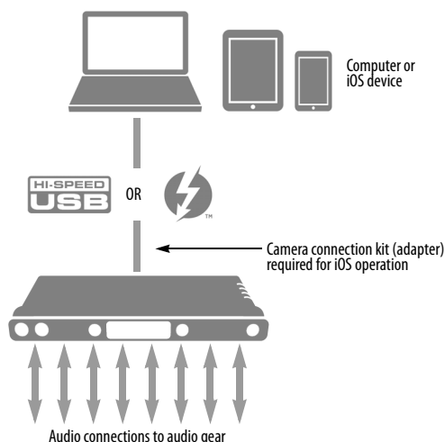
Figure 6-2: Using the 828es as an audio interface.
