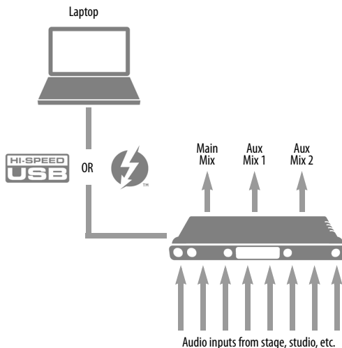
Figure 6-4: Using the 828es as an audio interface and mixer, simultaneously.
