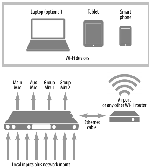
Figure 6-3: Using the 828es as a stand-alone mixer. This example demonstrates how you can control the mixer from several Wi-Fi devices.
