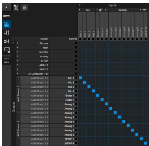
Figure 5-11: Routing physical inputs to the Mac.
