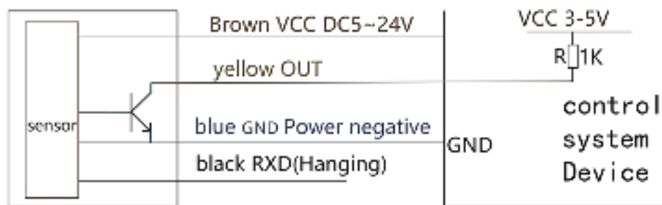
High and low signal output: wiring method to connect to controller or MCU
