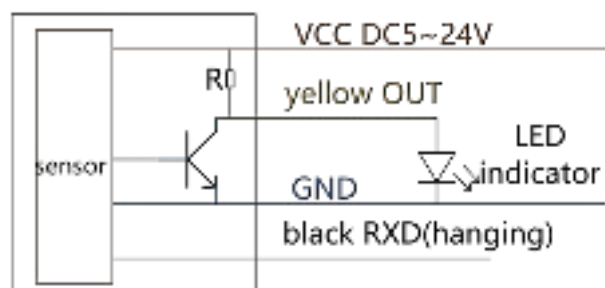
High and low signal output: Wiring method for connecting LED indicator
