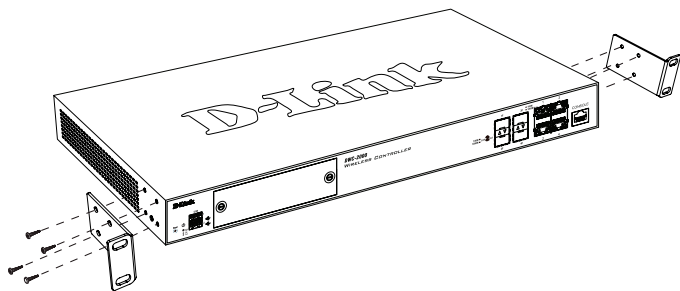
Figure 5. Supports de fixation
