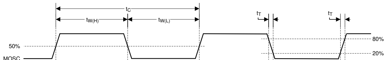
Figure 6-5. System Oscillators
