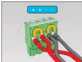
wiring: daisy-chained to next unit
