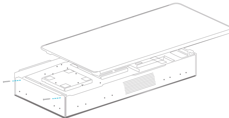
Figure 4: Removing the gateway cover
