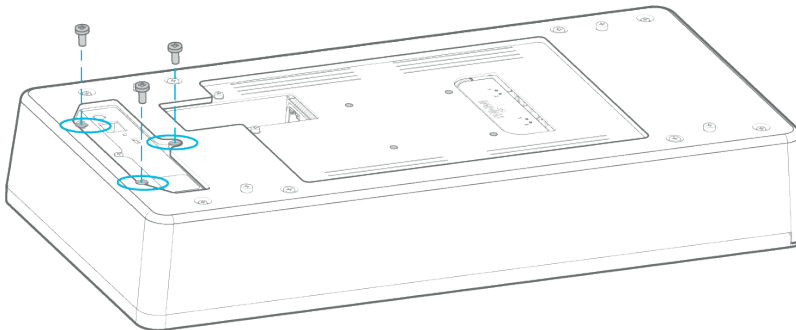
Figure 6: Securing the Radar
