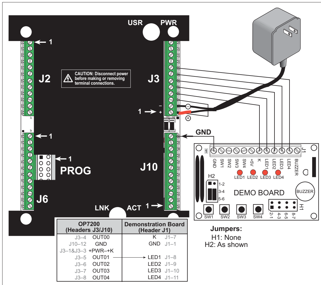
Figure C-2. Connections Between OP7200 and Demonstration Board for DIGOUT . C Sample Program
