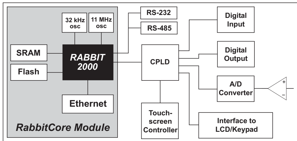
Figure 5. OP7200 Subsystems
