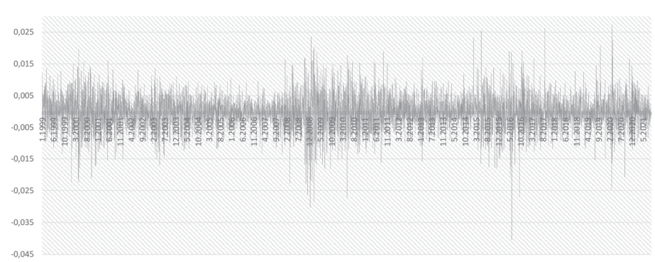
Figure 8. Log returns of the exchange rate for Croatian Kuna against the Great British Pound
