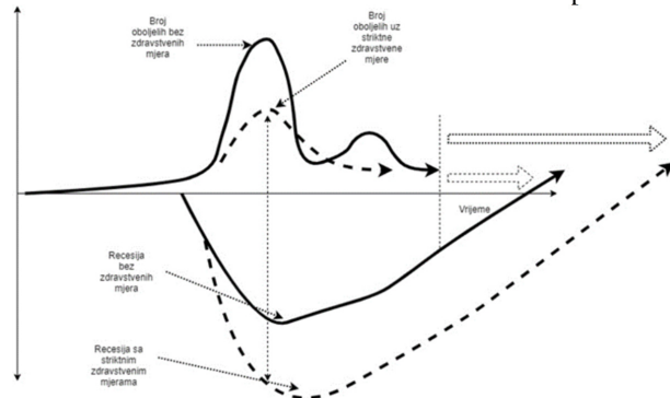
Picture 2. The theoretical curve of the COVID-19 pandemic and the recession curve
