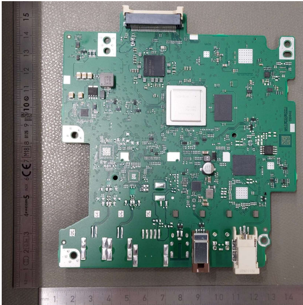
PCB 2 – Top
