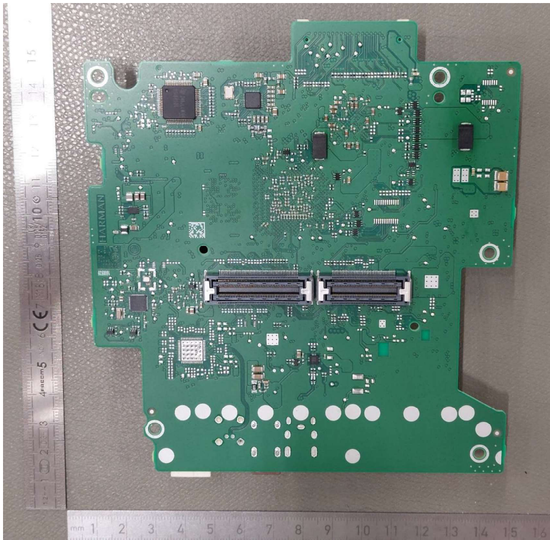
PCB 2 – Bottom
