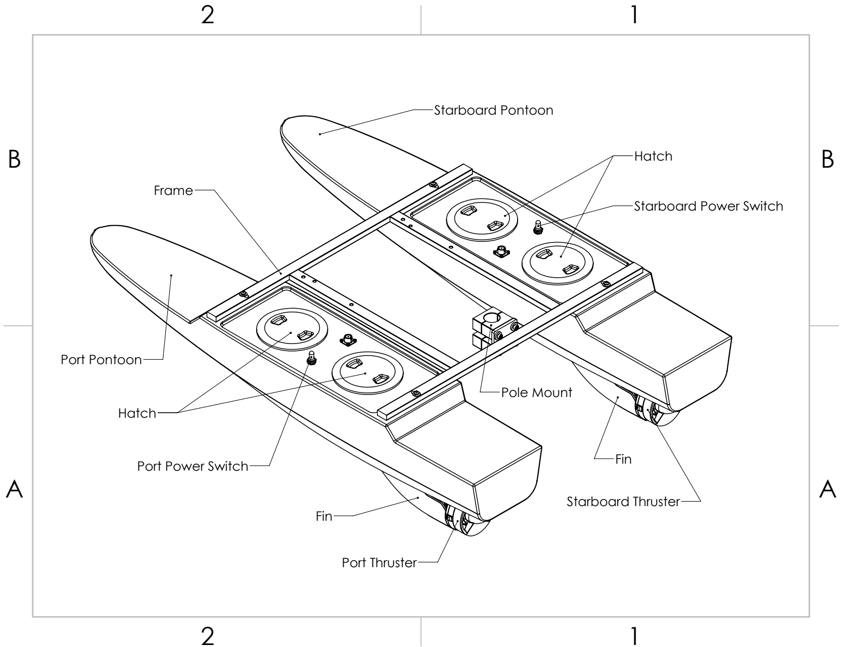
Figure 1: Hydroner™ RCV System Overview
