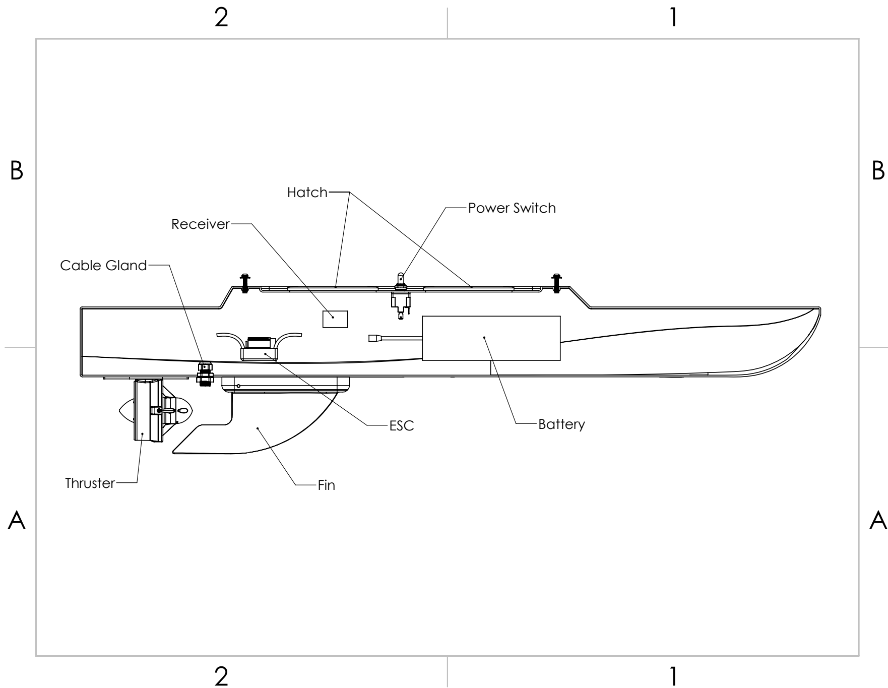
Figure 3: Hydroner™ RCV Side View
