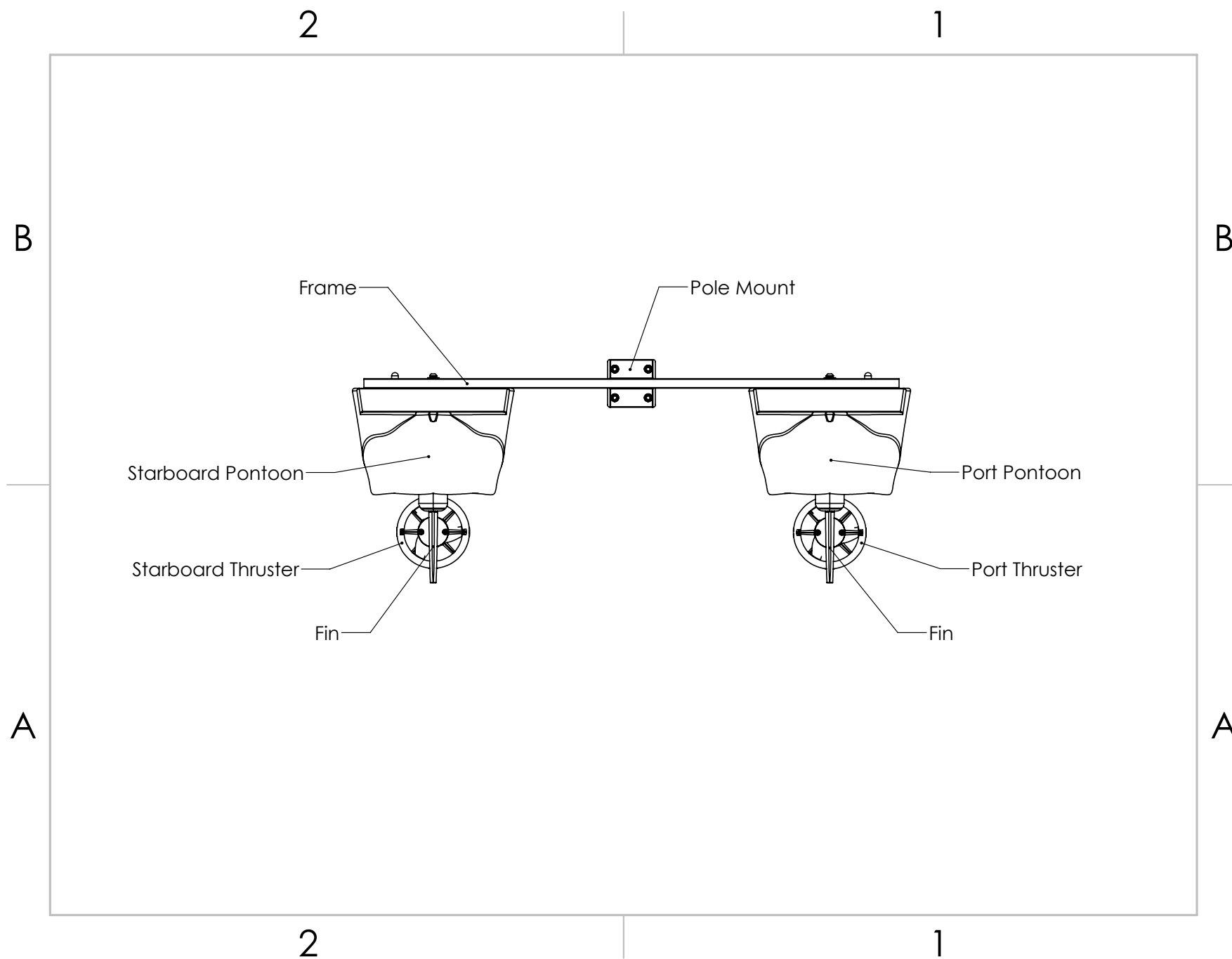
Figure 2: Hydrone™ RCV Front View
