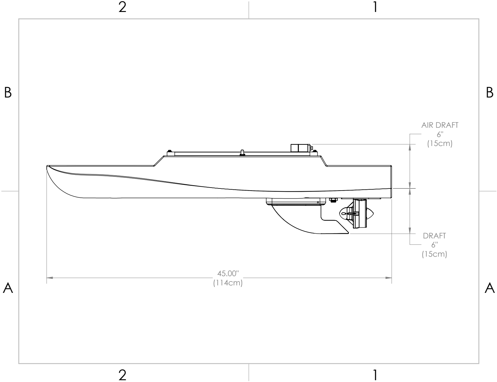
Figure 71: Side View Diagram
