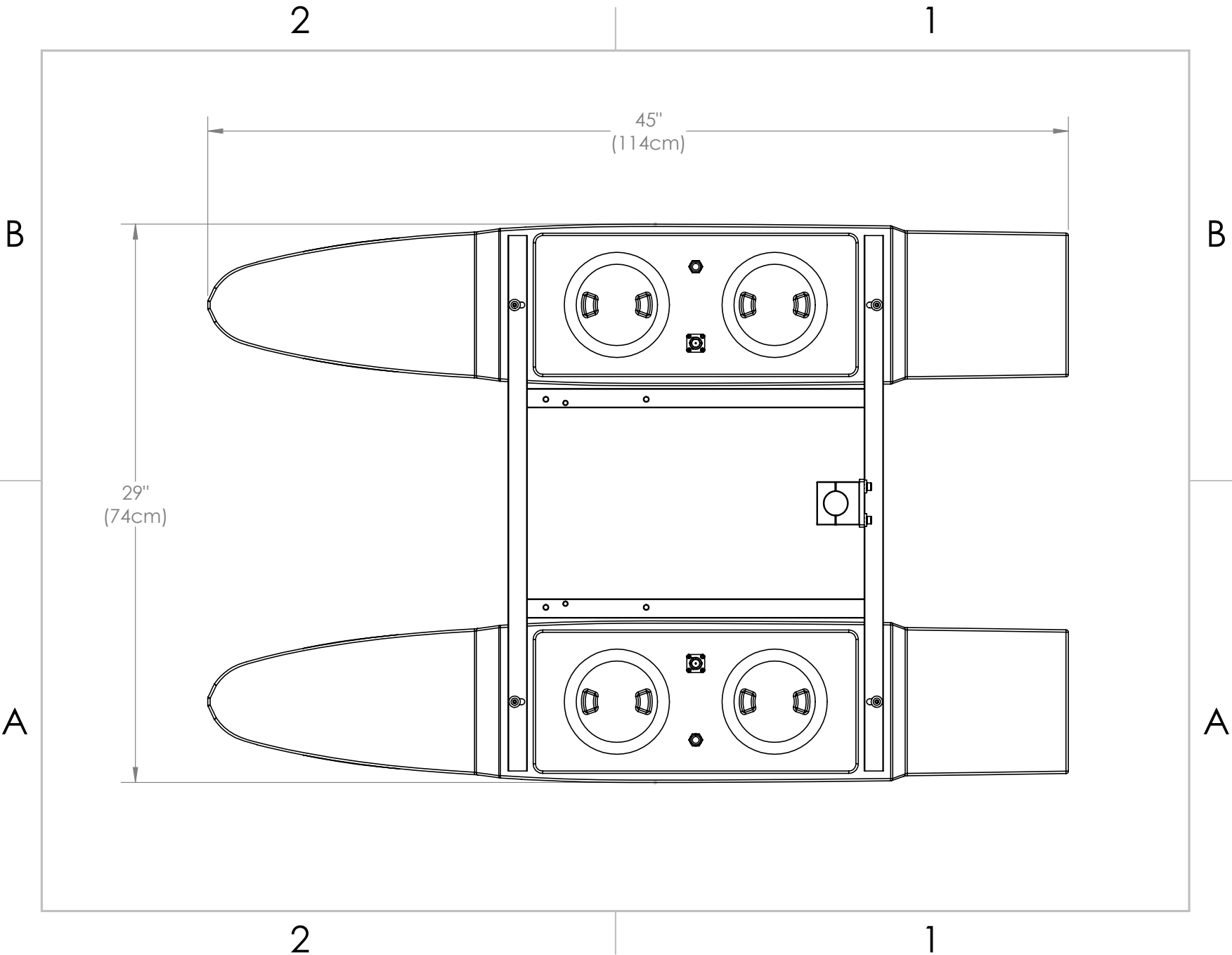
Figure 73: Top View Diagram
