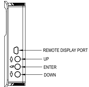
Figure 5: Side view of transmitter
