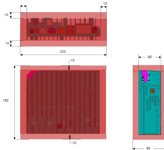
VCU Mandatory (Minimum) Thermal Keep-Out Zone
