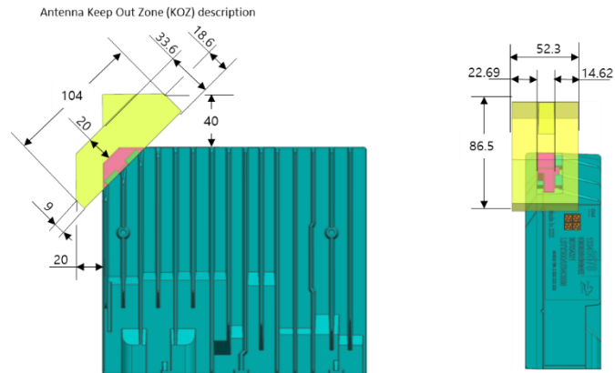
VCU Antenna Keep-Out Zone
