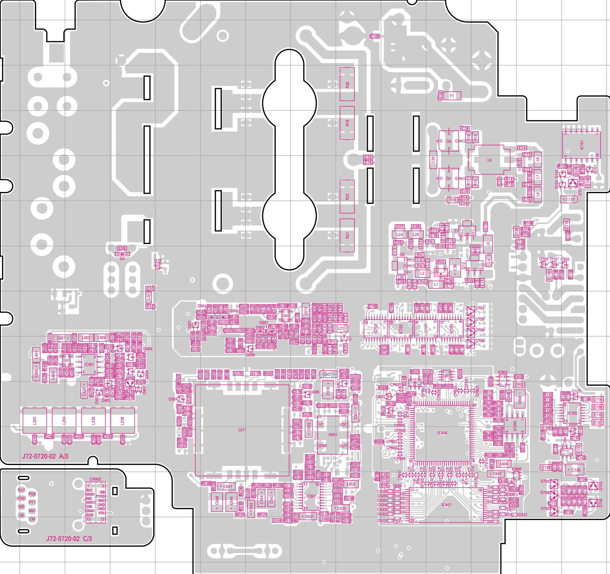
TX-RX UNIT (X57-6100-XX) (A/3, C/3) -10 : K -11 : K2 Foil side view
