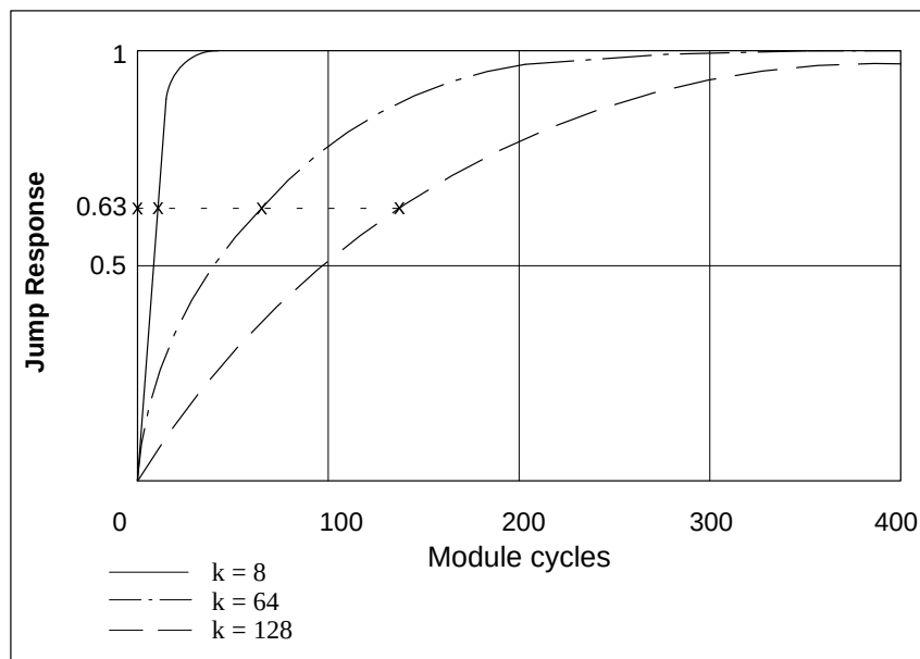
Figure 12-18 Jump response
