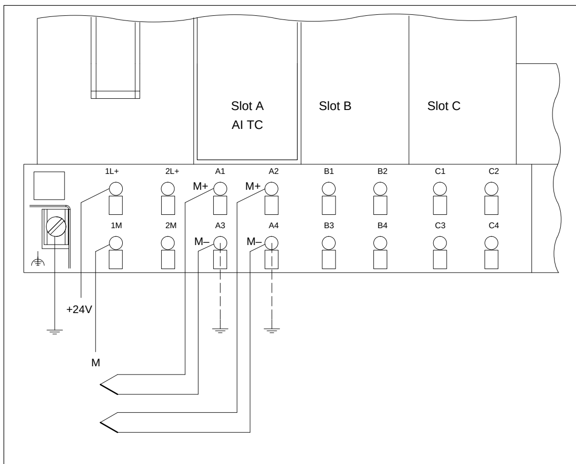
Figure 11-2 Connecting Insulated Thermocouples Without Compensation, With Internal Compensation, or Use of the Reference Temperature (Example TB 16SC)
