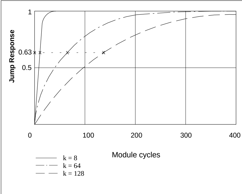
Figure 12-12 Jump Response
