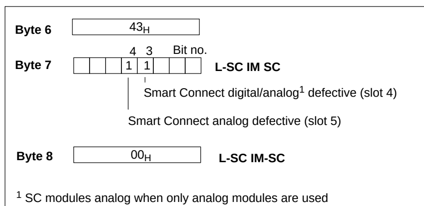
Figure 5-3 Structure of the Module Diagnosis with the COM/S7 Configuration Software for the ET 200L-SC IM-SC
