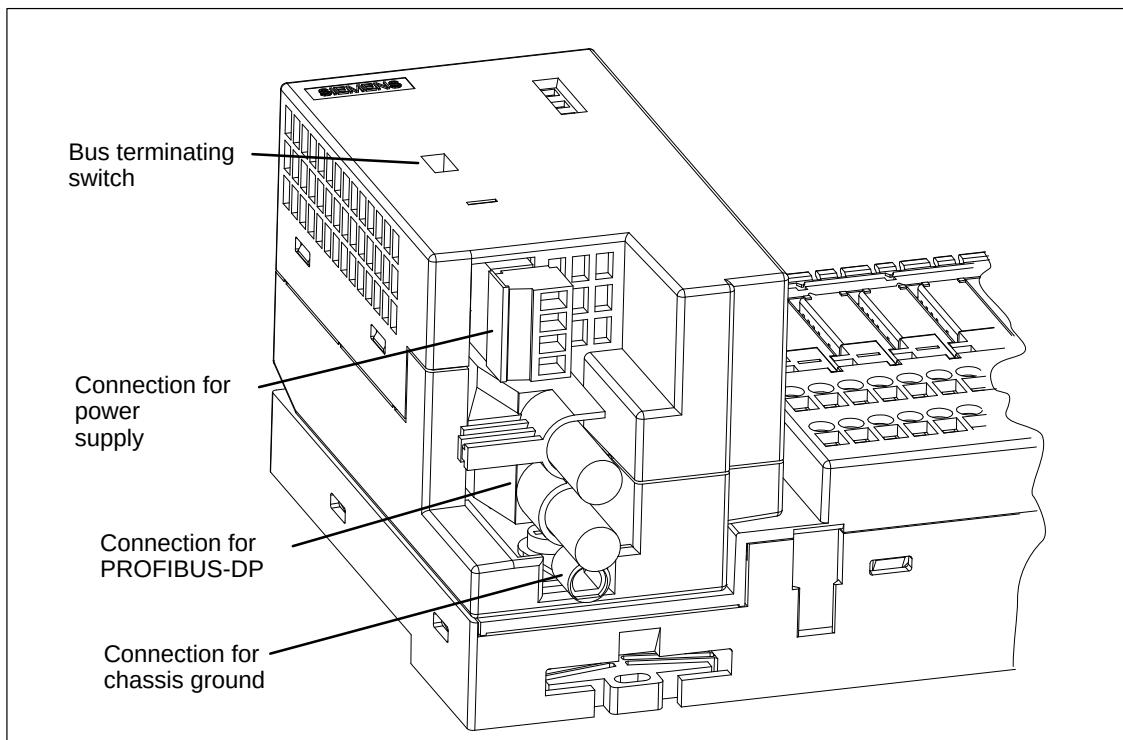
Figure 3-9 Connections of the IM-SC Interface Module
