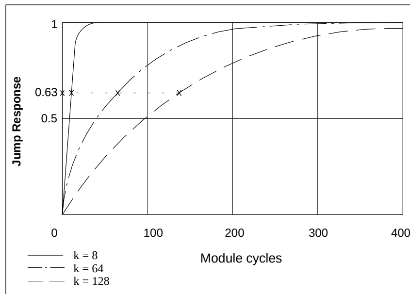
Figure 12-6 Jump response
